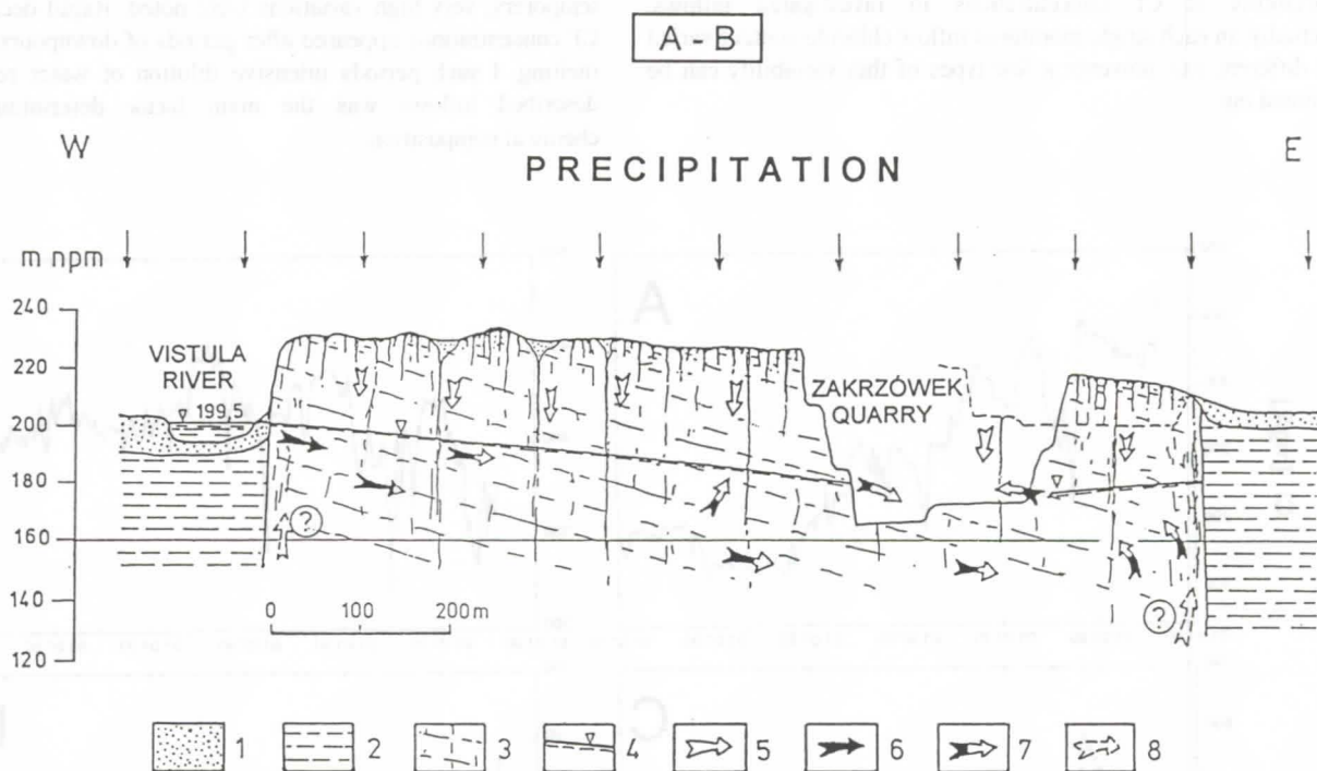
Fig. 4. Hydrogeological cross-section A-B. 1- sands, 2- clays, 3-limestones, 4- theoretical piezometric level, 5- fresh water (precipitation), 6- salt water from Vistula river, 7- mixed water, 8- ascending water.
