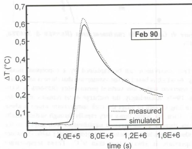
Figure 9: Model validation
