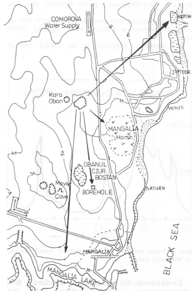
Figure 1. Hydraulic connections determined using radioactive and activable tracers in South Dobrogea karst system.
