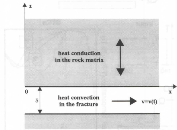
Figure 1: Conceptual model of flow and heat transport in a single fracture with constant aperture
