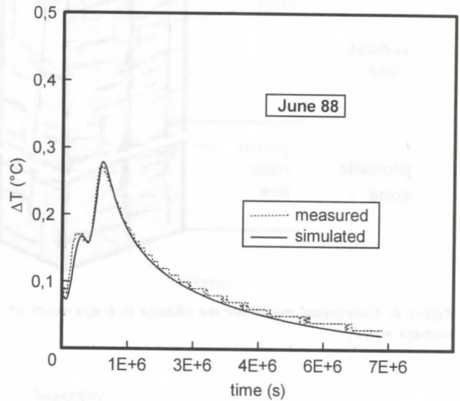
Figure 7: Model calibration with respect to spring water temperature
