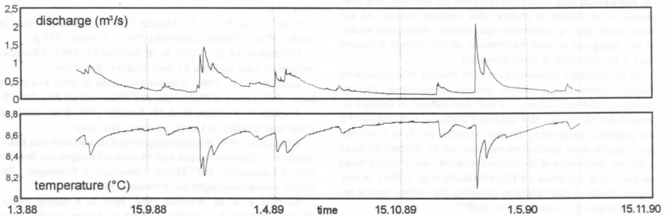
Figure 5: Spring water temperature and discharge at the Gallusquelle karst spring
