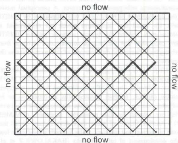
Figure 2: Geometry of the conduit system in the lower layer of the model domain. The initial diameters of the tubes connecting row 9, 10 and 11 are 1 mm and of the remaining tubes 0.4 mm.
