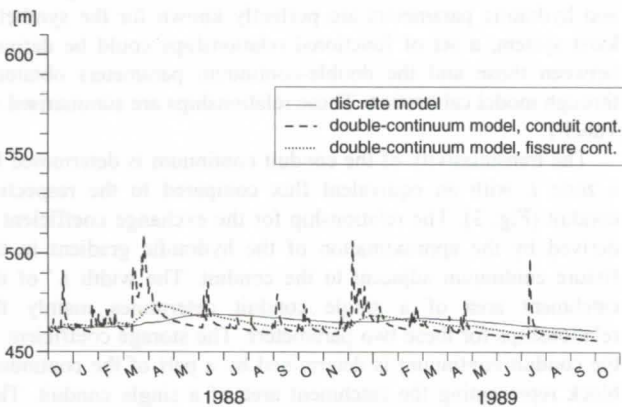
Figure 4: Spring discharge and piezometric head time series at the measurement points P1, P4 of the calibrated double-continuum model.
