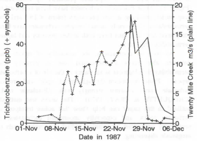
Figure 4. Rapid changes in trichlorobenzene concentrations in a dolomite aquifer in Ontario, showing lagged inverse correlation to runoff.
