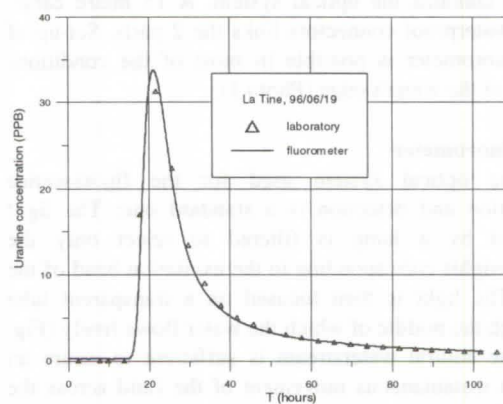
Fig. 2 a & b: Comparison of the results from the fluorometer (line) and the sampler (triangles) at 2 sites.
