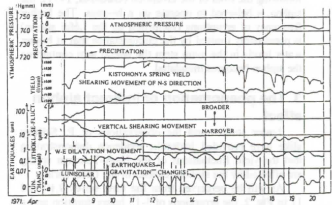
Fig. 7. Lithoclase fluctuation registered in the Vass Imre cave. The time series are following: Atmospheric pressure, precipitation, Kis-Tohonya spring yield, shearing movement of N-S direction, vertical shearing movement, W-E dilatation movement, earthquakes, lunisolar gravitation changes. (April, 1971)
