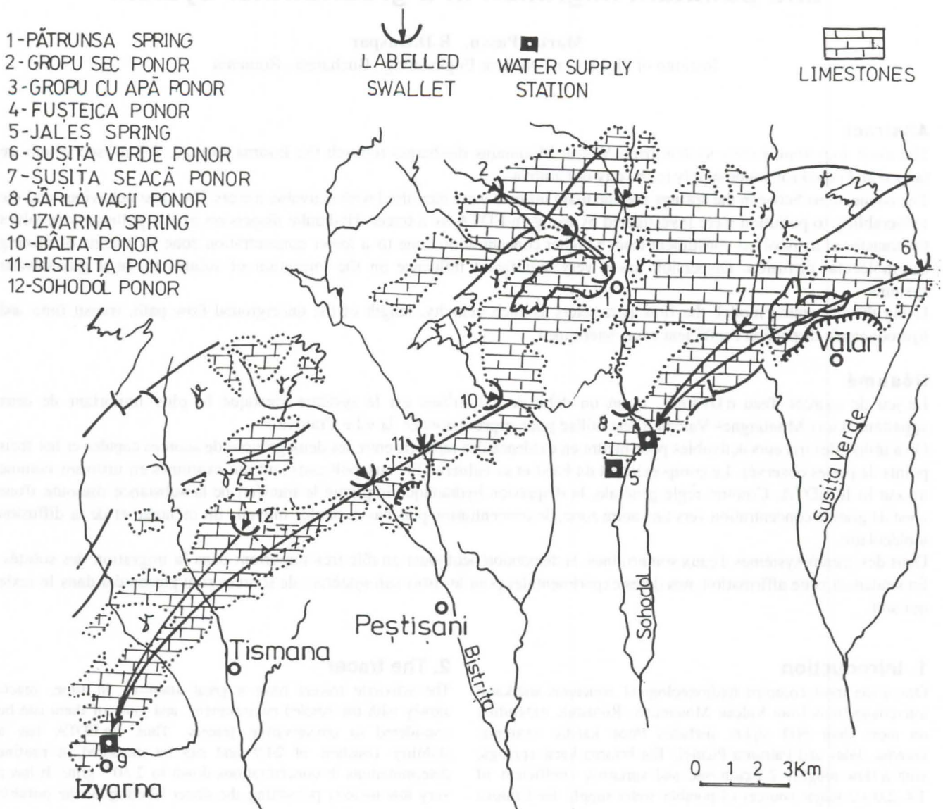
Figure.1. General sketch of Southern Valcan Mountains karst.
