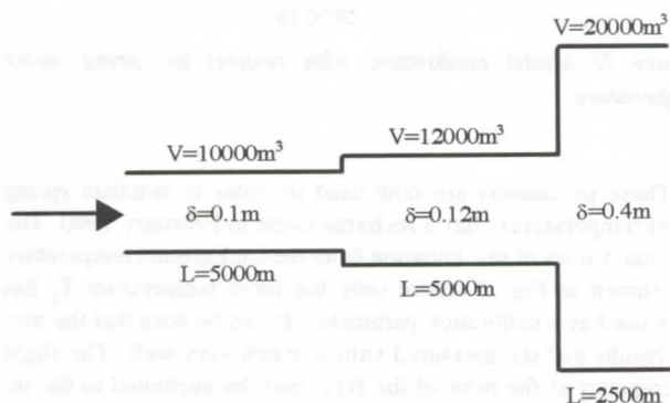
Figure 8: Equivalent fracture for the Gallusquelle karst catchment
