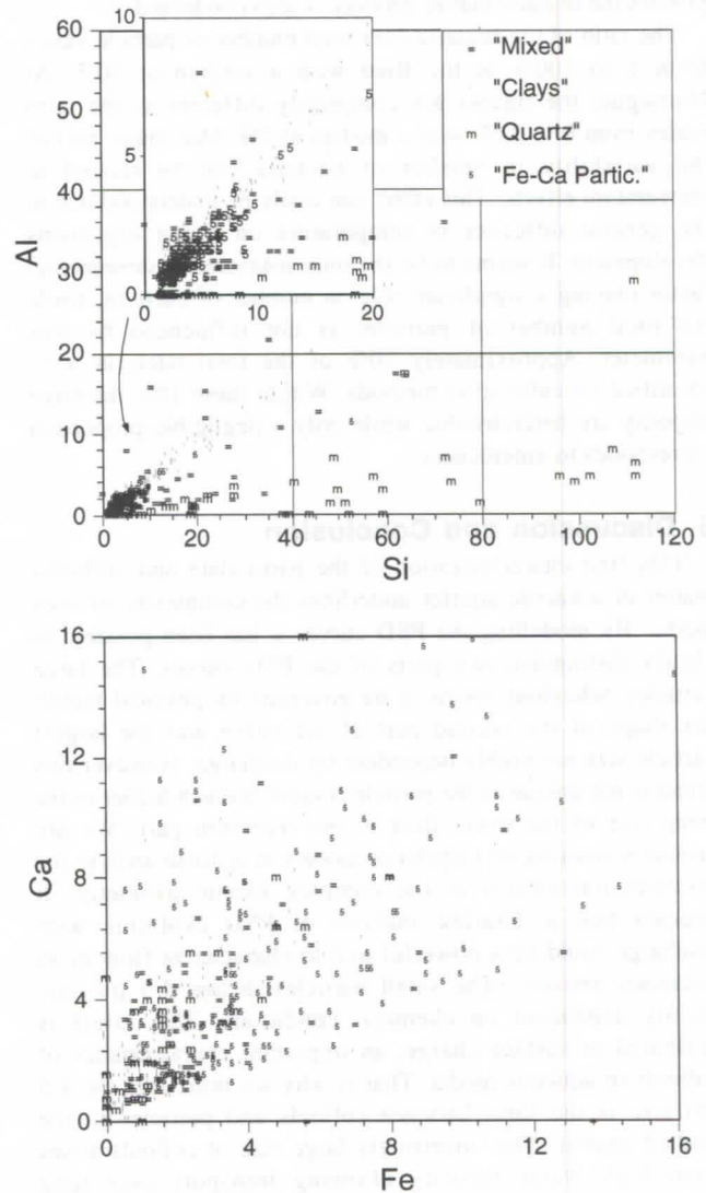
Fig. 4: SEM-EDS intensities (relative units) measured on particles from the Bied brok: a) Si and Al, b) Fe and Ca
