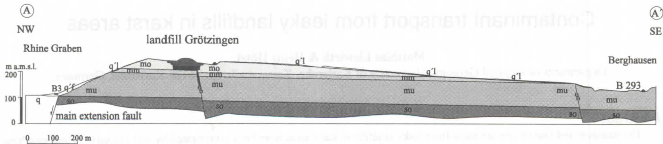
Fig. 2: Geological cross section A-A' as indicated in Fig. 1. (q, q', q'1 = Quaternary sediments, mo = Upper Muschelkalk, mm = Middle Muschelkalk, mu = Lower Muschelkalk, so = Upper Buntsandstein).
