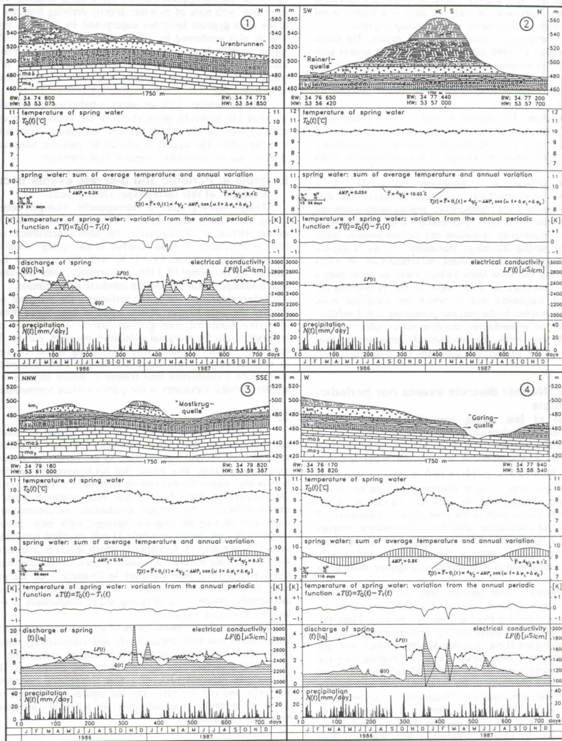
Fig. 2: Spring examples 1 to 4: • Cross-section through the main inflow area of the springs (above). The three diagrams set out below describe temporal temperature changes in the spring water: represented are: • the measurement series as discrete values of the actual temperature progression T_0(t) ; • the primary (annual) harmonic \theta_1 (periodic change with amplitude AMP_1 ) obtained by Fourier analysis from T_0(t) , representing (together with the mean annual temperature T ) the measurement values of periodic progression T_1(t) ( \Delta\phi_0 indicates the phase difference between earth's surface and spring water temperature; \Delta\phi_1 the phase difference of the earth's surface temperature referred to January 1st); and • the deviations \Delta T(t) of the measurement values from the periodic progression T_1(t) . These describe the temperature progression freed of periodic behavior, resulting from short-lived events. Both lowermost diagrams show • spring discharge Q(t) and • electrical conductivity LF(t) for spring water and for • local precipitation N(t) .
