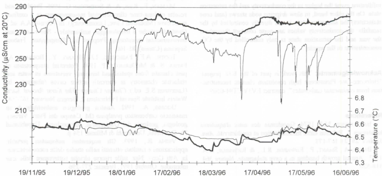
Figure 4.: Combined conductivity and temperature (daily running mean) records for G1 (bold lines) and G2 (thin lines) stalactites. Note that conductivity of G1 dripping is generally over 10\ \mu\text{S}/\text{cm} higher than that of the fast dripping G2.
