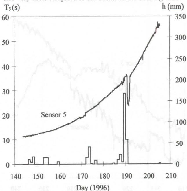
Figure 2: Recording of the flow rate of sodastraw 5, from May 28 th to July 24 th 1996 showing the swelling feature of July 8 th . T_s (in s) is the mean time between two drops, averaged over 3 minutes. T_s is then inversely proportional to the flow rate. Rain data (h in mm) are from the Autrans meteorological station.
