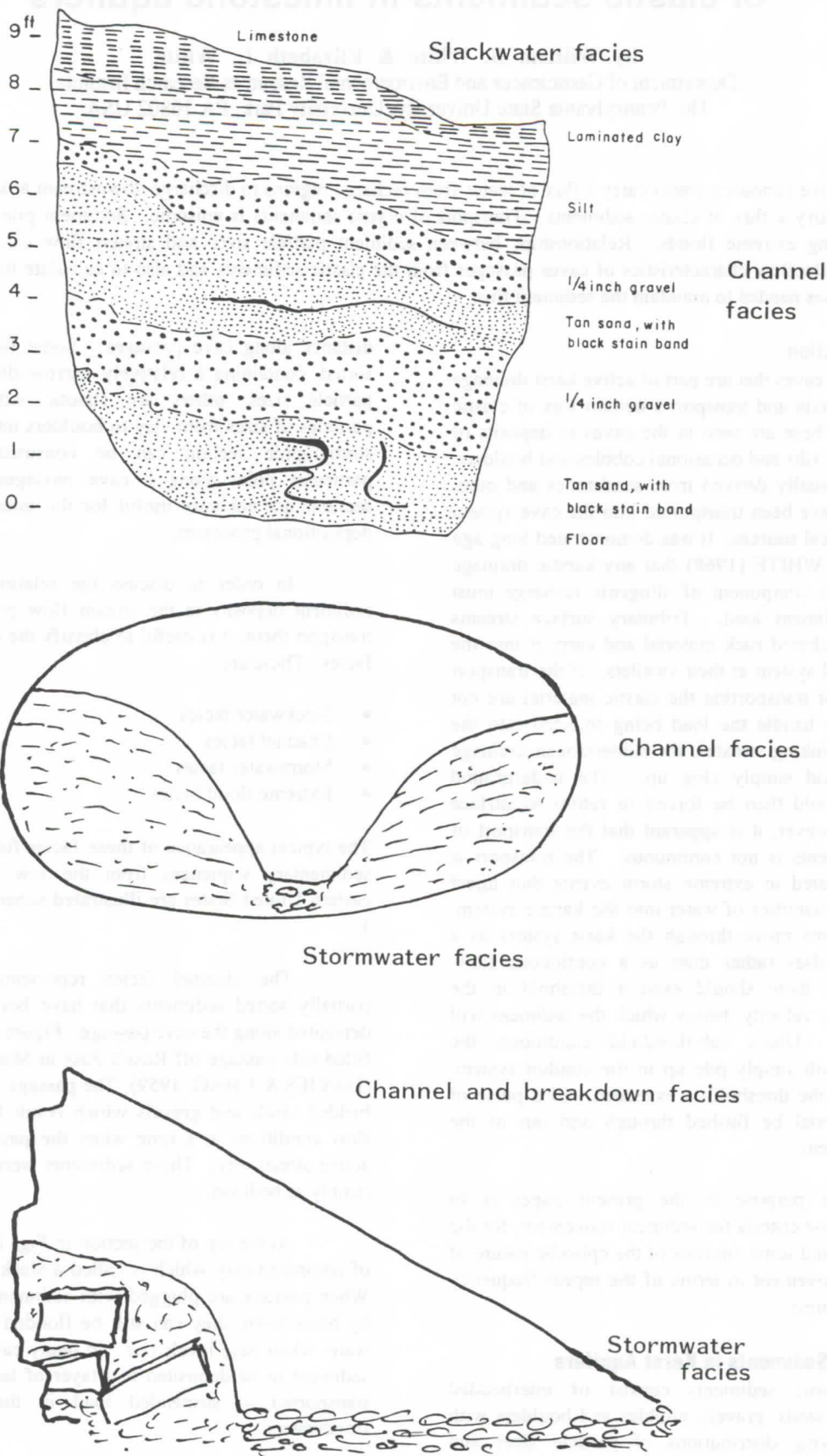
Figure 1. Sketches showing clastic sediment facies: (A) Mammoth Cave (from DAVIES & CHAO, 1959), (B) Generic channel form, (C) Tytoona Cave, Pennsylvania, USA
