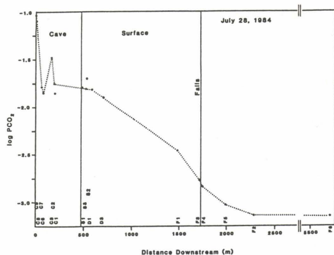
Figure 2. \log P_{\text{CO}_2} for water samples versus distance along the flow path. The thermal spring inside Warm River Cave is taken as the start of the flow path (0 m).
