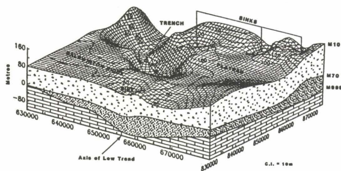
Fig. 5. Block diagram of the Poundmaker depression area (courtesy of G. S. Jones, Husky Oil). Scale in meters. M10 -top of the Mannville; M999 -pre-Cretaceous unconformity; M70 -an intra-Mannville marker.
