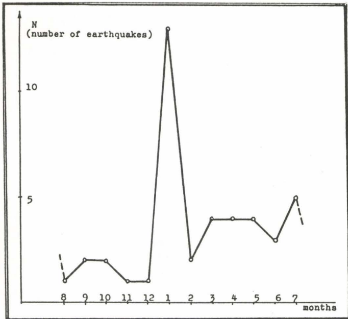
Fig. 7. Heavier earthquakes frequencies diagram in epicentral region of Biokovo from 1901 to 1970.
