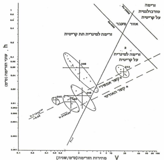
Fig. 6: Film flow dynamics in shafts, Ofra Reynolds Number (Re) calculated for water temperature-10°C. h. film flow thickness (cm) 2. super-critical laminar flow v. flow velocity (cm/sec) 3. empiric function 1. sub-critical laminar flow 4. theoretic function
