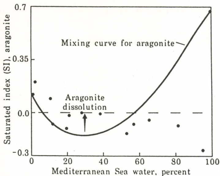
Fig. 3. Aragonite saturation index plotted as a function of percentage Mediterranean Sea water. Points are observed values of groundwater samples, and the line is a calculated conservative mixture.
