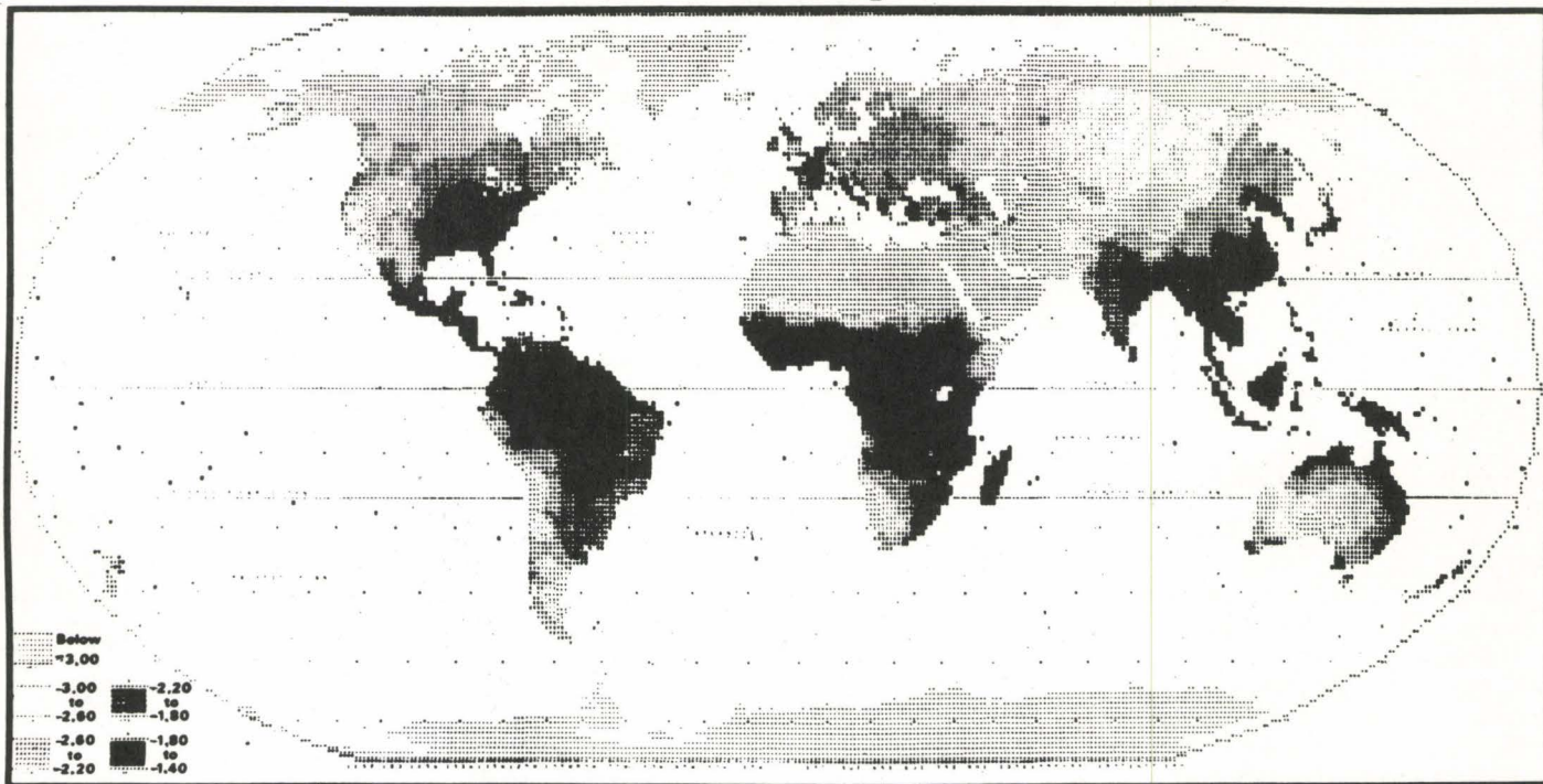
Fig. 2. The predicted global pattern of mean growing-season soil log (PCO 2 ) (after Brook, 1983).
