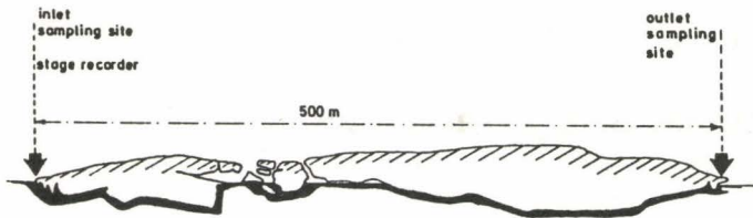
Fig. 2. Vertical, longitudinal section of the cave. Flow from left to right. Surveyed by cave diving, the middle entrances possess characteristics of truncation by glaciers in the past.
