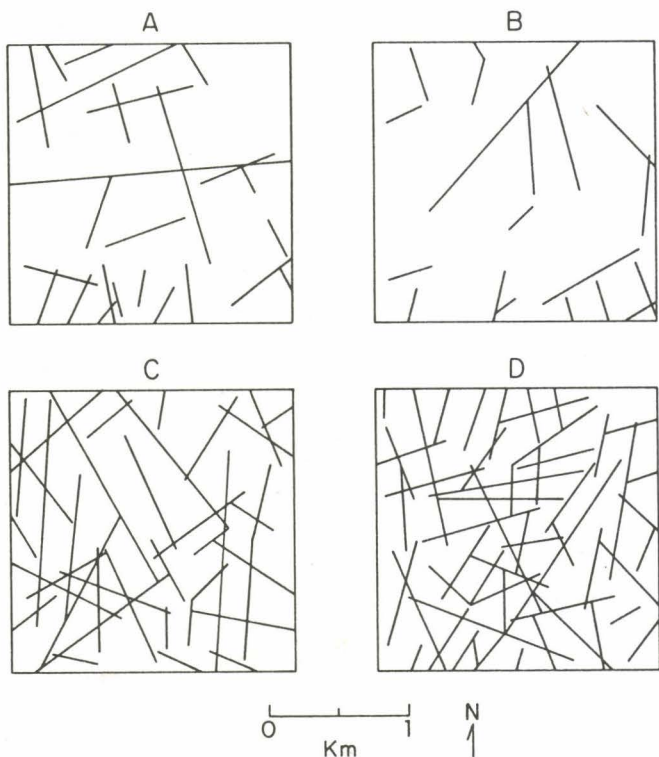
Fig. 2. Fracture Traces in Areas A-D.
