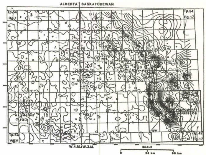
Fig. 2. Structural configuration of the top of the Mannville, a second order residual surface. Contour interval 10 m. The main «salt» collapse belt is identified by a dashed line (A-A). Lines marked SW-NE and N-S indicate the orientation of structural cross-sections shown of Fig. 4 and 7 respectively.
