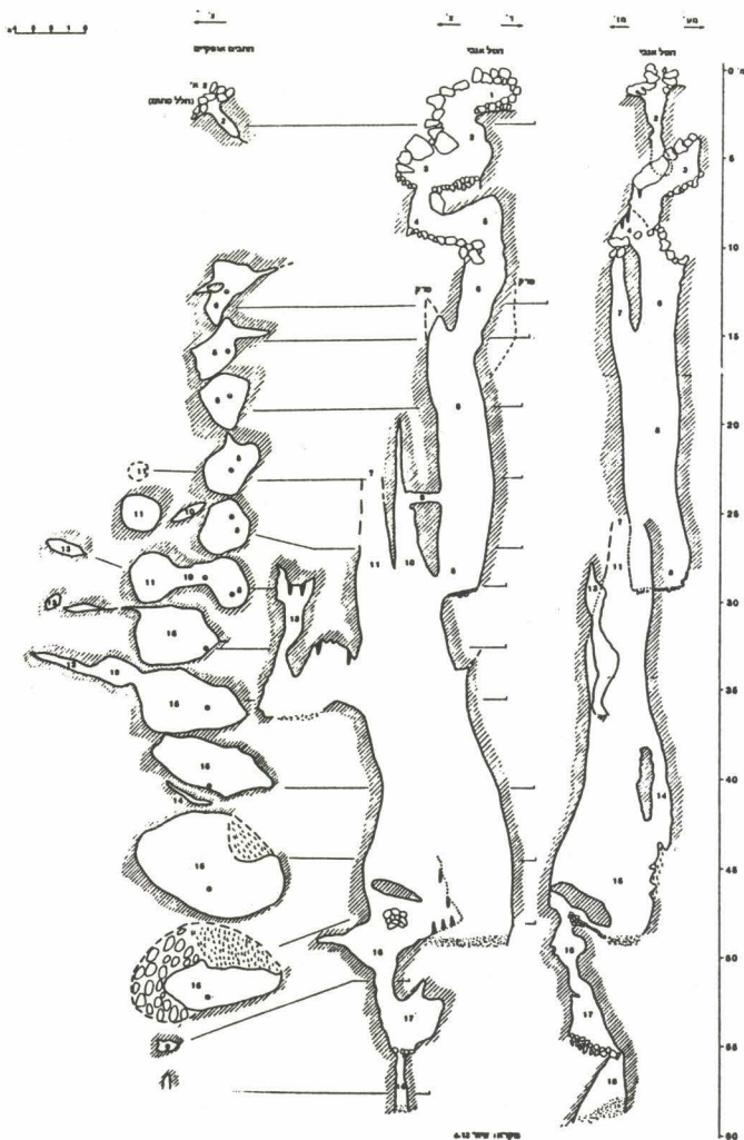
Fig. 3: The «Chinese Pothole» in Ofra, vertical and horizontal sections, survey: A. Frumkin, ICRC. BCRA grade 5D
