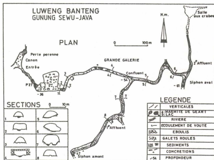
Figure 3. Plan de Luweng Benteng.
