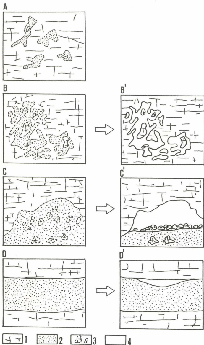
Fig. 1. Development of cavern in disaggregated carbonate rocks. A-B-C-D various stages of disaggregation B',C',D' caverns, 1- solid lithified carbonate rocks, 2- disaggregated carbonate rocks, 3- relics of lithified carbonates, 4- empty caverns. Modified after, Dzulynski, Sass-Gustkiewicz, 1985.
