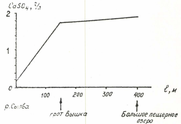
Fig. 3. Change of \text{CaSO}_4 content depending on the distance from the water edge of the Sylva River during high water period in 1974 (data by V. S. Lukhin and E. P. Dorofeev)
