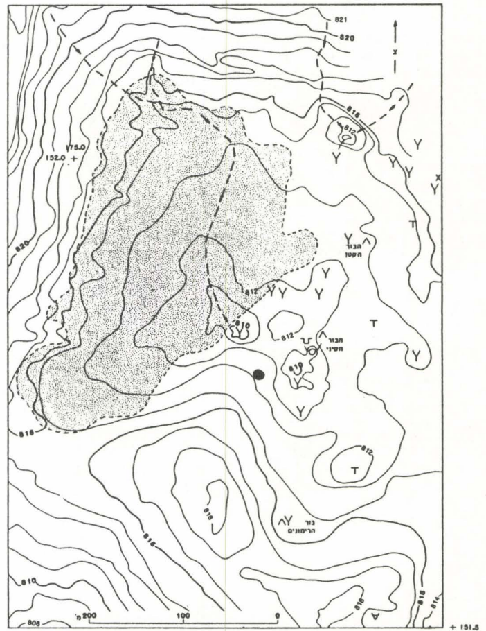
Fig.2: Karst phenomena in northern Ofra plateau
