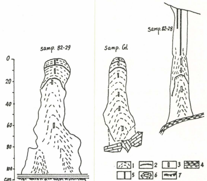
Fig. 2. Locations of subsampling for U-series dating of three stalagmites. 1. Growth veins in stalagmites; 2. depositional interruptions; 3. locations of subsamples; 4. travertine; 5. straw stalactite; 6. breakdown rock pieces; 7. clay.
