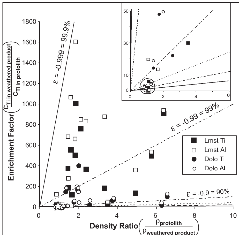
Figure 3: Enrichment factors for the insoluble element Ti are plotted against density ratio for oxide layer and punk rock samples. Samples from both limestone (squares) and dolostone protoliths (circles) are shown; the unaltered protolith plots at 1 (star) for both limestone and dolostone. The data for Al (open symbols) is also plotted. Various degrees of strain ( \epsilon ) are plotted as lines originating from the origin. Positive strain represents dilation and negative strain, collapse. Inset: Expanded origin corner showing clustering of punk rock samples (circled).
