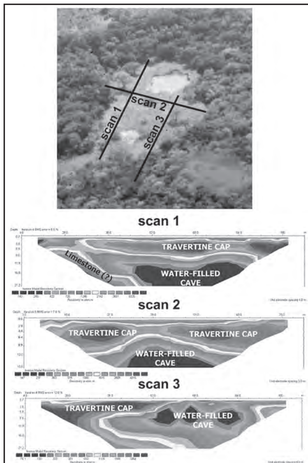
Figure 2: ERI surveys conducted at the cenote La Pilita were conducted in 2003 to test the applicability of the geophysical method to image this karst setting. Direct access to the water-filled cave in this cenote verified that the ERI data represented actual features that are hypothesized in other fully capped cenotes.
