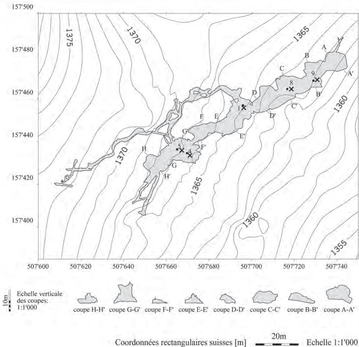
Figure 3: Measurements undertaken with U-GPS 1 at the Grande-Rolaz cave. The shift observed between the control points and the position estimated by U-GPS 1 let us expect that U-GPS 1 is more precise than the cave survey (systematic error of about 2 to 3 meters).
