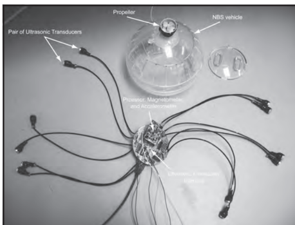
Figure 2: Prototype sensor node circuit assembly and enclosure.
