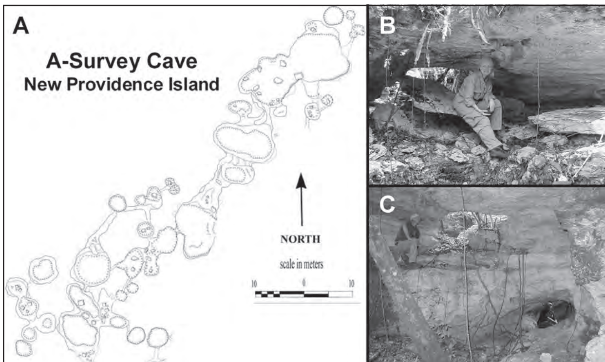
Figure 3: A-Survey Cave, New Providence Island, Bahamas. (A) Map of A-Survey Cave, a series of interconnected chambers (modified from Mylroie et al., 2008). (B) Phreatic chamber of A-Survey Cave, truncated by collapse. (C) Large chamber in A-Survey Cave, with passages both high and low.
