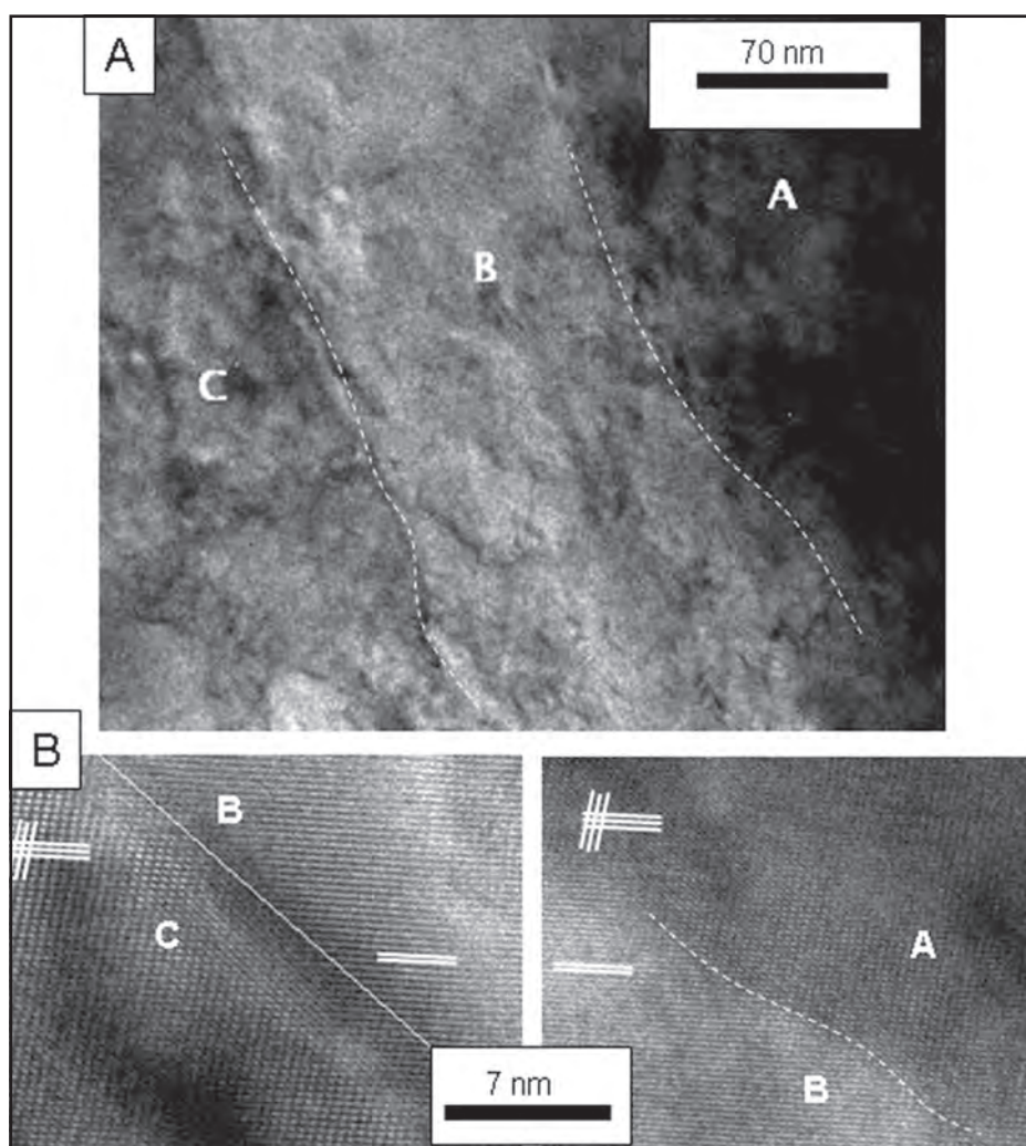
Figure 4: HRTEM images of a region of the soda straw calcite. Differences in contrast represent subtle nano-scale imperfections of the atomic ordering. Top image shows three regions of phase contrast defined by dotted lines. The images on the bottom show that regions A and C show lattice fringes in two directions, while region B shows lattice fringes in one direction, yet all three regions show lattice continuity in one direction indicating they are all part of the same crystal. These subtle differences are interpolated to propagate as crystal defects such as split crystal growth.
