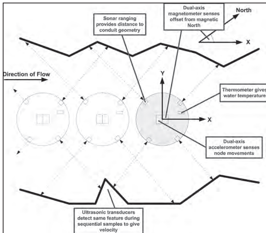
Figure 1: Neutrally buoyant sensor – Conceptual operation (plan view).
