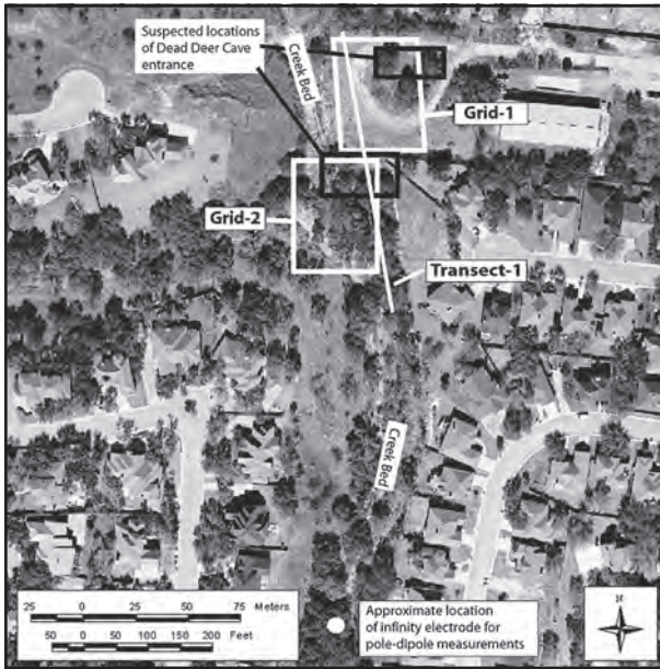
Figure 2: Locations of electrical resistivity transects and grids occupied at suspected locations of Dead Deer Cave.
