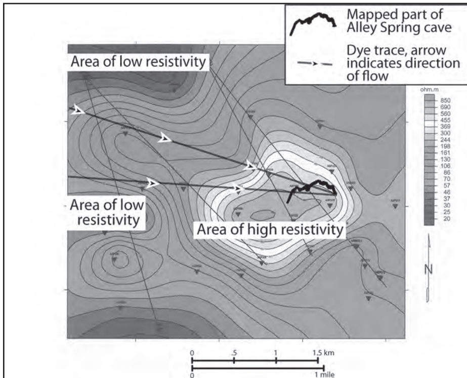
Figure 7: Subsurface electromagnetic resistivity map and structural contours in the vicinity of Alley Spring. Resistivity map generated at the 160 meter elevation (525 foot) (above mean sea level). See Figure 4 for vertical relationship to the Alley Spring Cave.
