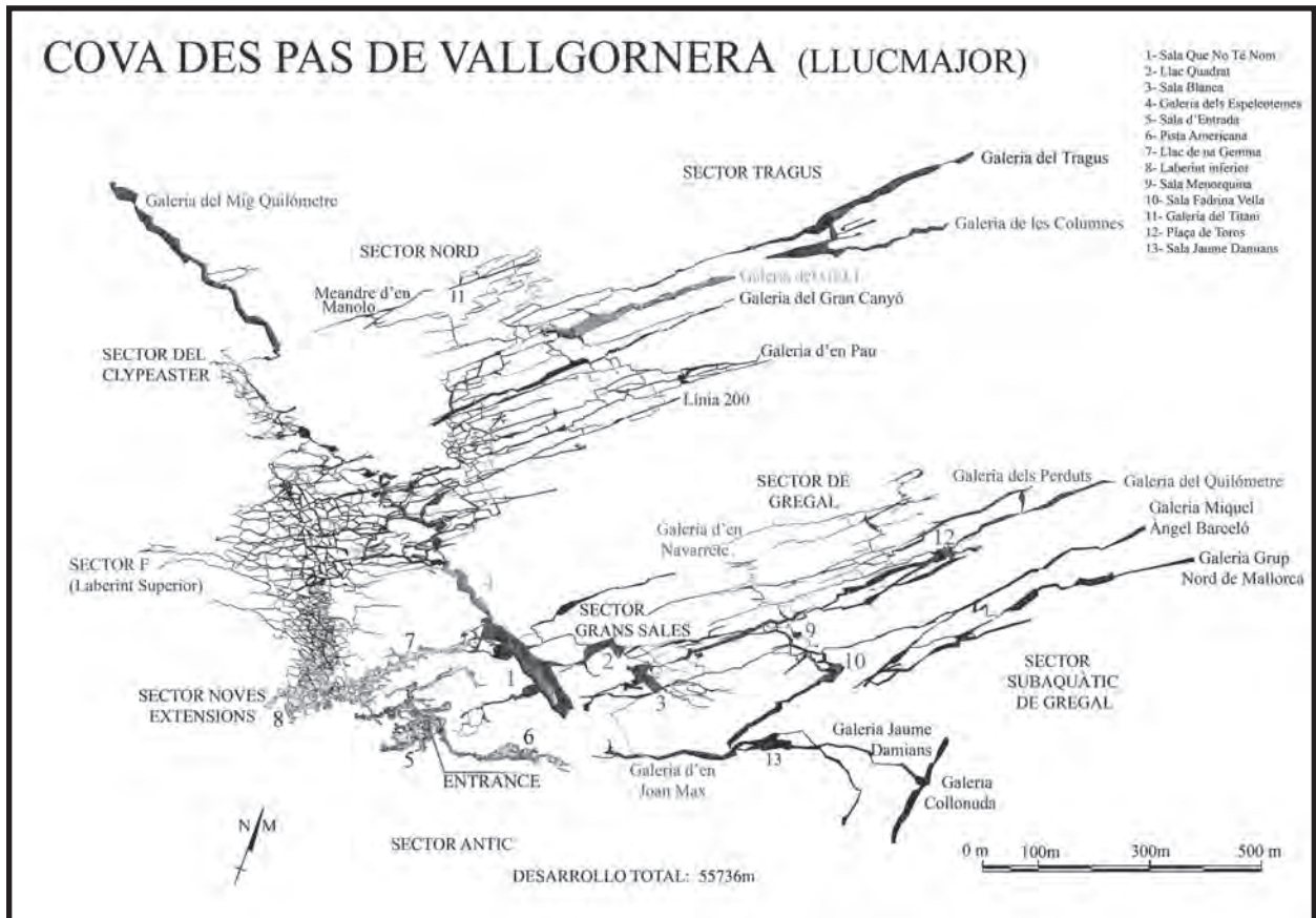
Figure 2: Survey of the cave with the main sectors identified.
