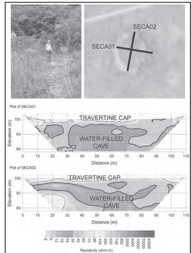
Figure 3: Upper left photo shows the setting electrodes in Posa Seca, and the upper right zoomed-in aerial view shows the perpendicular geometry of the two transects surveys at this site. ERI processed images shown below of these two transects show a clear electrical distinction between the thin travertine cap on the surface and an apparent water-filled cave underneath.
