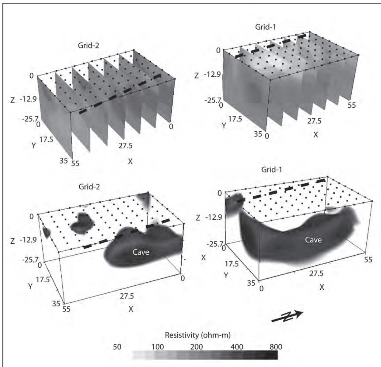
Figure 4: Block models of x-slices and volume rendering of inverted resistivity for pole-dipole measurements collected at Grid-1 and Grid-2. The block models are positioned to show the south to north variation in subsurface electrical resistivity beneath the surveyed areas. Dashed lines represent the placement of Transect 1.
