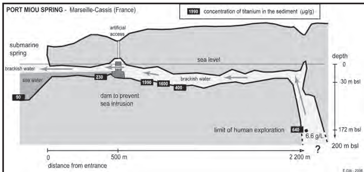
Figure 1: Cross section of the Port Miou gallery.
