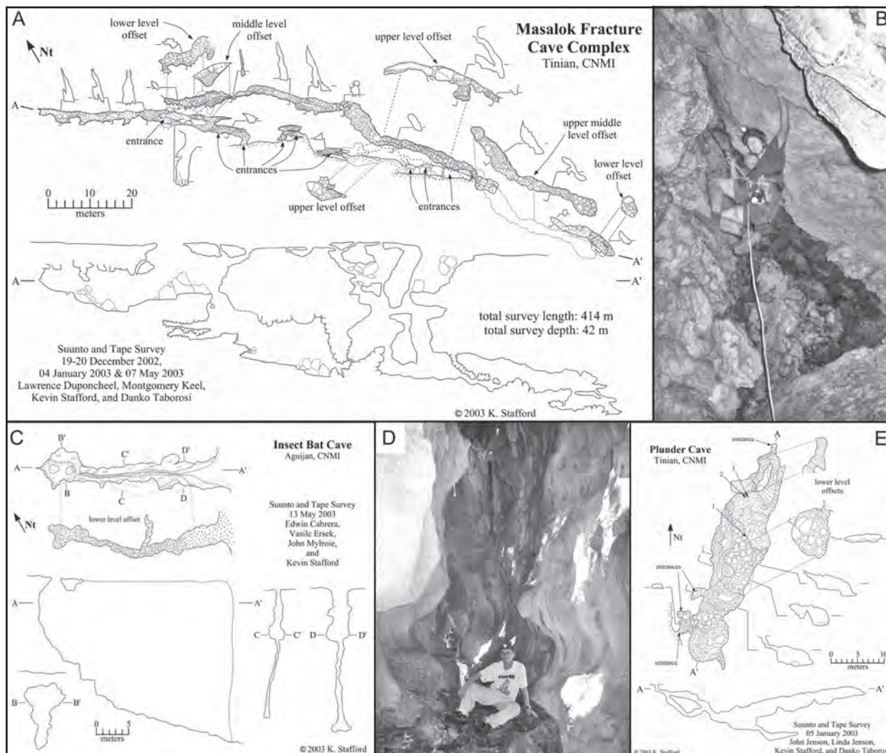
Figure 6: Fissure caves associated with bank margin failures tend to be laterally extensive (A), nearly vertical (B) and can reach significant depths (A). Fissure caves associated with tension-release fractures extend inland perpendicular to scarps (C) and often show horizontal widening (D) associated with increased dissolution from the mixing of spring discharge on seawater. Fissure caves developed along faults (E) often show horizontal widening when intersecting the water table (maps from Stafford, 2003).
