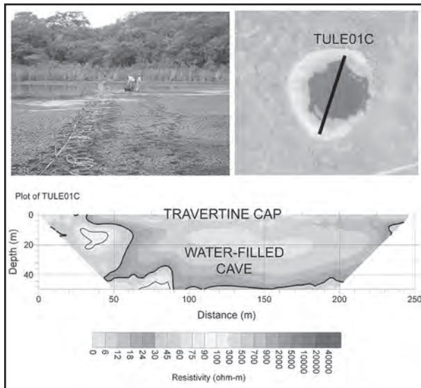
Figure 4: The upper left photograph on the cap of Tule and the ERI instrumentation. . The upper right aerial photo shows the ERI transect location. Note that water is present (about 1 meter deep) at the time of this photograph. Water levels were lower because of period of little rain at the time it was geophysically imaged, but the floor was wet and saturated. The lower image shows results from the survey. Electrodes were spaced at 5-meter intervals to span the 250 meter cenote, and the thin travertine cap is faintly resolved in this dataset. It is possible that a lower floor of the water-filled cave could be present, although the data in this spatial range are not optimal for geologic interpretation.
