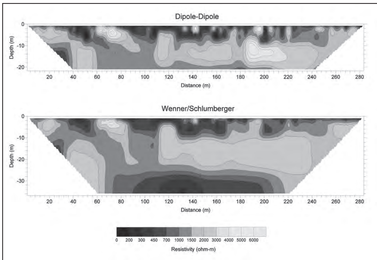
Figure 1: Vertical cross sections of electrical resistivity collected with a dipole-dipole array (top) and a Wenner/Schlumberger array (bottom). Lower resistivity is denoted by dark colors and is interpreted to be shale- or marl-rich limestone. Higher resistivity is denoted by light colors and is interpreted to be massive limestone. The highest resistivity is denoted by white and is interpreted to be potential solutional cavities.
