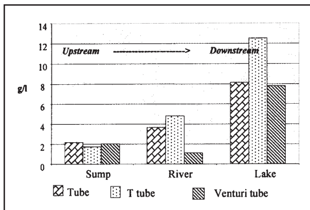
Figure 4: Sediment trapped in sump, in river and in lake with different models of trap.
