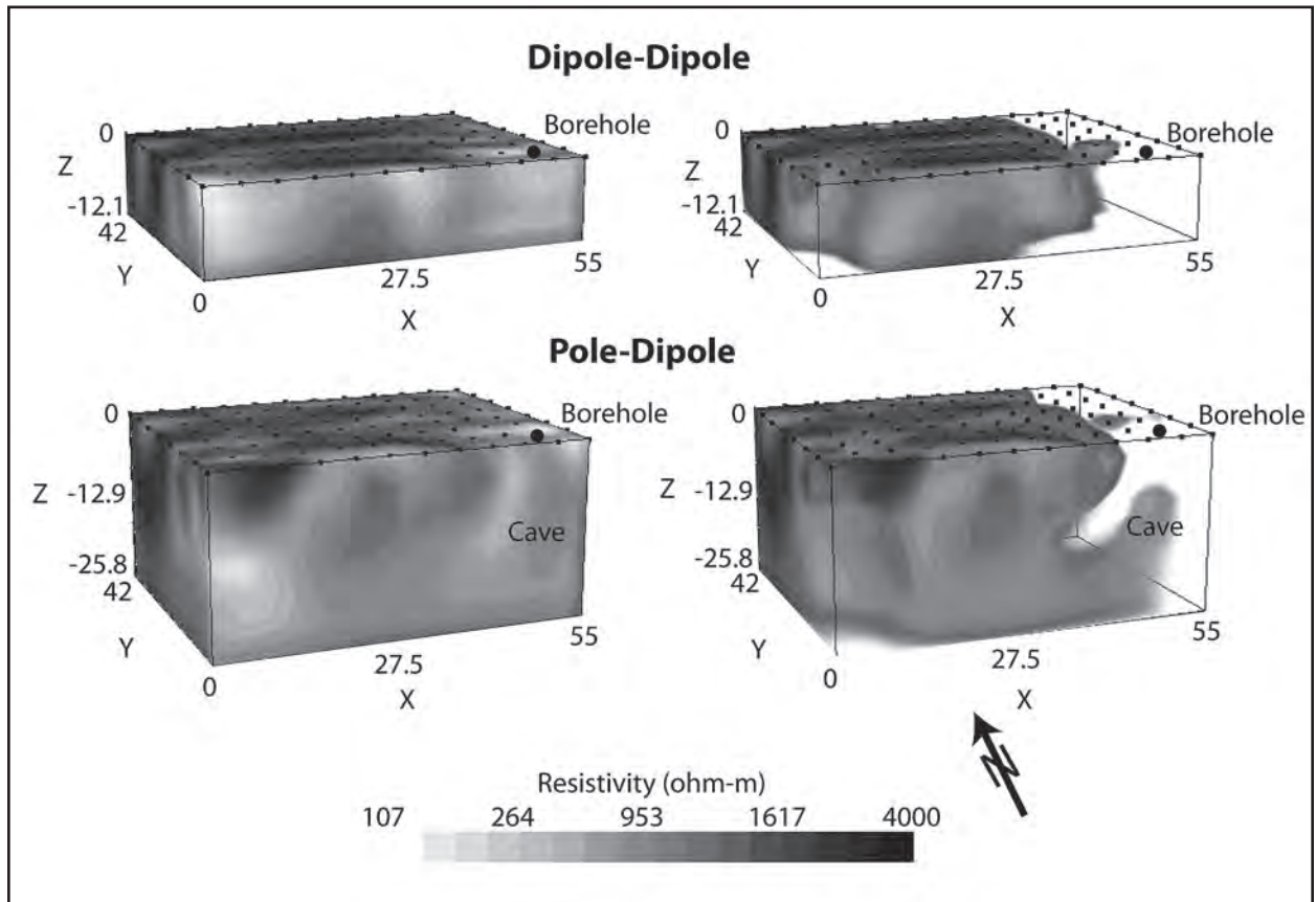
Figure 5: Block models and volume rendering of inverted resistivity for dipole-dipole and pole-dipole measurements collected at site in northern San Antonio, TX. The block models are positioned to show the west to east variation in subsurface electrical resistivity beneath the surveyed areas.
