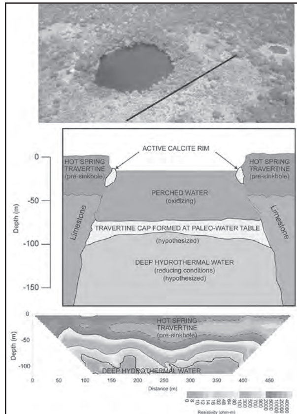
Figure 5: Top photo shows the cenotes Verde (left), La Pilita, (right), and a portion the location of the ERI transect line conducted near Verde. This photo shows the radially inward travertine growth at La Pilita. The middle image graphically displays the hypothesis that a paleo-water table once existed below the present day water table, allowing for a travertine cap to form. Subsequent rise in regional water levels creates a perched water body above this flooded cap. ERI data from the Verde transect (bottom image) shows evidence of the deep hydrothermal water hypothesized in the middle diagram.
