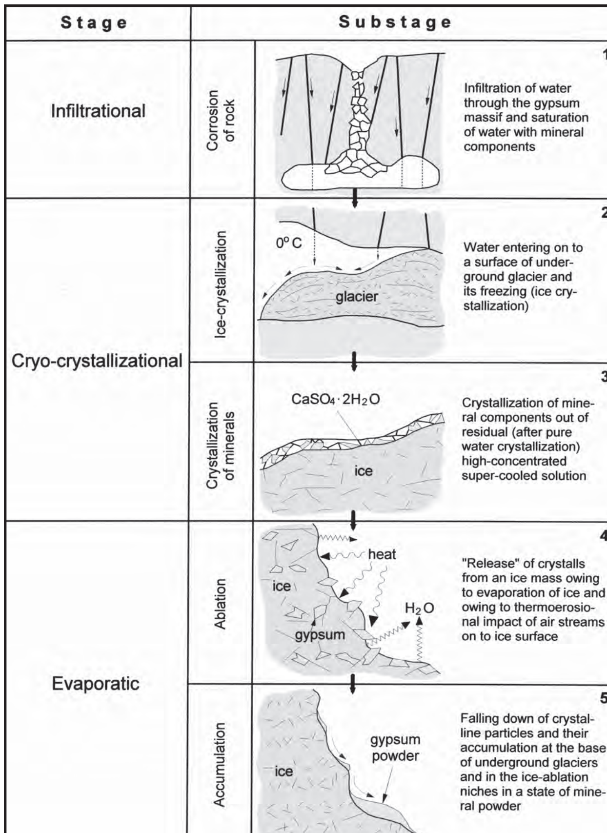
Figure 4. Main stages of formation of crychochemical gypsum powder under perennial ice in Koungur Cave (figures illustrating stages in different scales).
