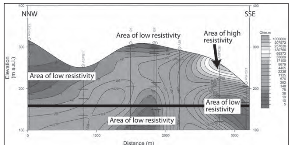
Figure 5: Audio-magnetotelluric and topographic profile line P-4. Location and elevation of cave is estimated from cave map and side view (Fig. 4). 3X vertical exaggeration. See Figure 5 for line and station locations.
