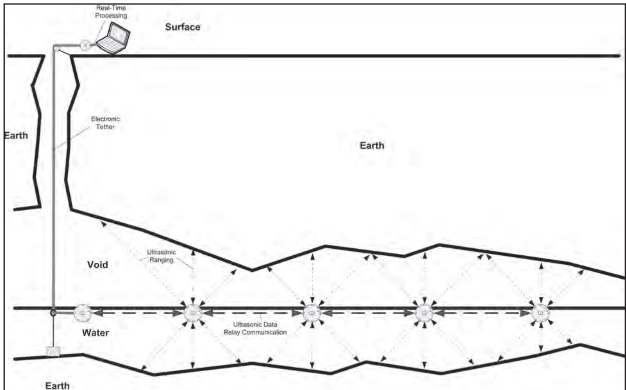
Figure 5. NBS data collection approach via an electronic tethered base station and multiple mobile units.
