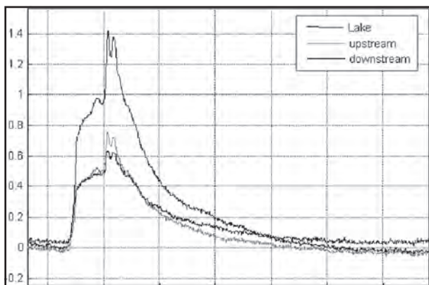
Figure 3: Water level in the lake, upstream and downstream sump during flooding.
