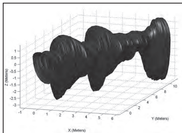
Figure 3: Final rendering of cave passage using sonar and magnetometer data collected during the July 3, 2008, prototype sensor deployment.
