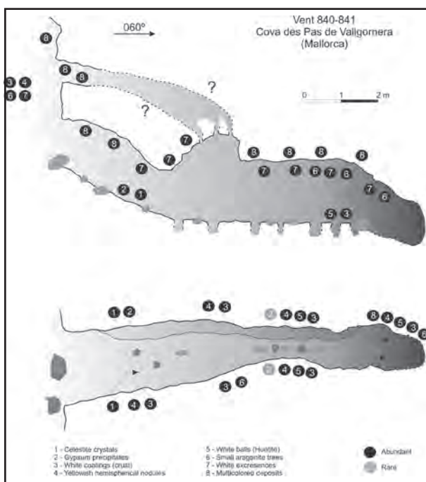
Figure 3: Vent sketch with the distribution of the main mineral facies present.
