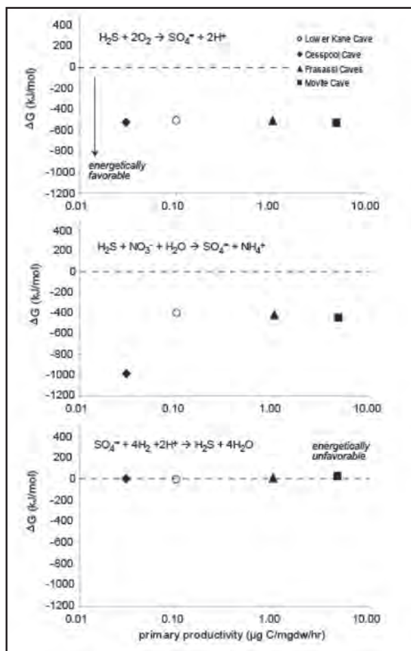
Figure 1: Free energies of various redox reactions.
