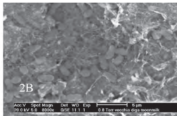
Figure 3: SEM photomicrographs of microbial cells intermixed with carbonate minerals from moonmilk in Grotta della Foos (1B), microbial cells from the moonmilk-water interface in Grotta della Vecchia Diga (2B).
