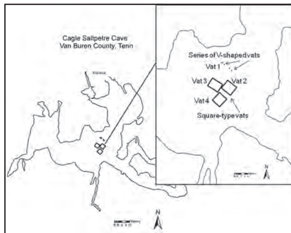
Figure 1: Plan view map of Cagle Saltpetre Cave, showing the locations of the V-shaped vats and square-type vats discussed in this study (from, BLANKENSHIP et al., 2009: Figure 2).
