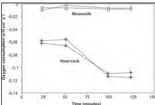
Figure 2: The decrease of oxygen concentration as microsensor tip approaches the sample was determined for moonmilk samples and host-rocks at four different incubation periods. The slope represents the consumption of oxygen by the sample with depth in a microchamber where oxygen diffuses in from the upper, open part while at the bottom the sample consumes the dissolved oxygen.
