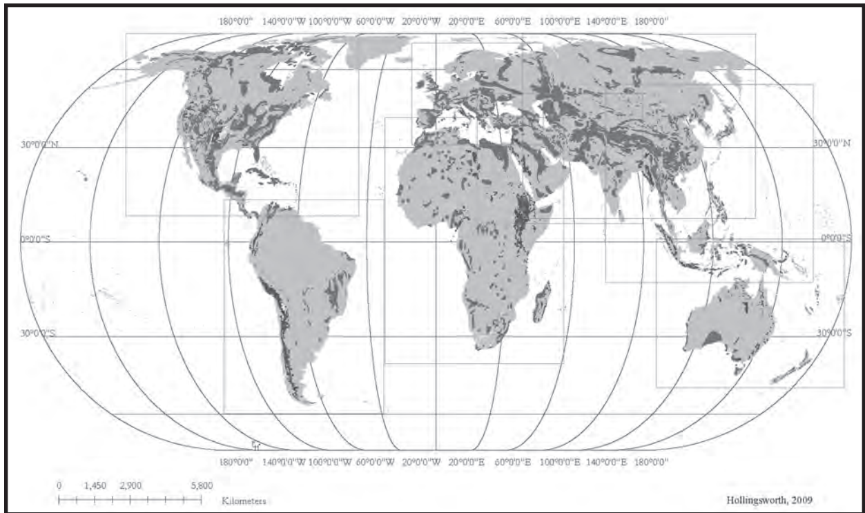
Figure 2: Map showing karst regions of the world (KROW) with regional-scale subareas delineated by rectangles. Land masses are shown in light gray, carbonate karst is represented as dark gray, evaporite karst is represented as white, and pseudokarst is represented as black (after Hollingsworth, 2009).
