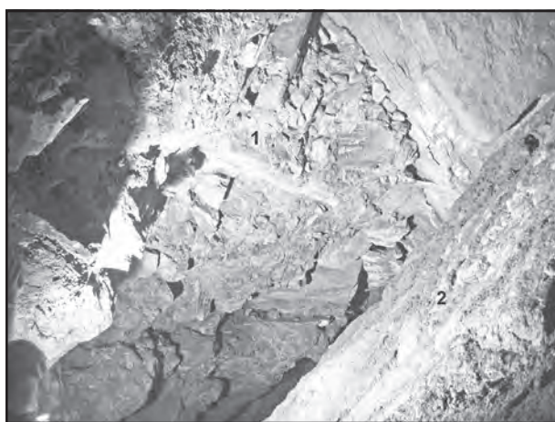
Figure 5: In the Name Chamber (Sterkfontein), the roof is constituted by two old breccias (1). A younger deposit forms a talus and has partially filled the chamber. This example shows how breccias are interpenetrated and often in stratigraphic inversion (L. Bruxelles).
