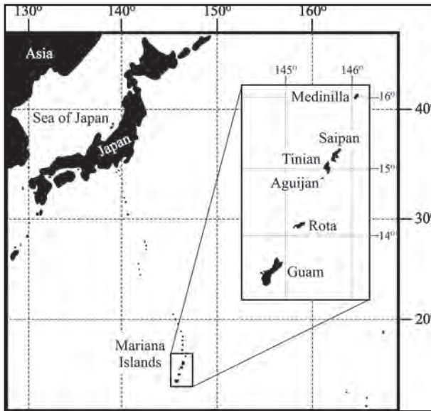
Figure 1: Map showing location of the Mariana Islands, with the six southernmost islands containing significant carbonate rocks shown expanded (adapted from Stafford et al., 2005).
