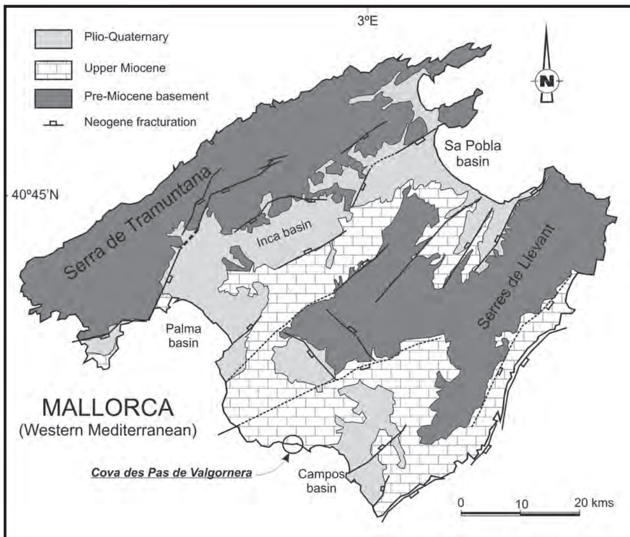
Figure 1: Simplified geological map of Mallorca Island showing the location of Cova des Pas de Valgornera.
