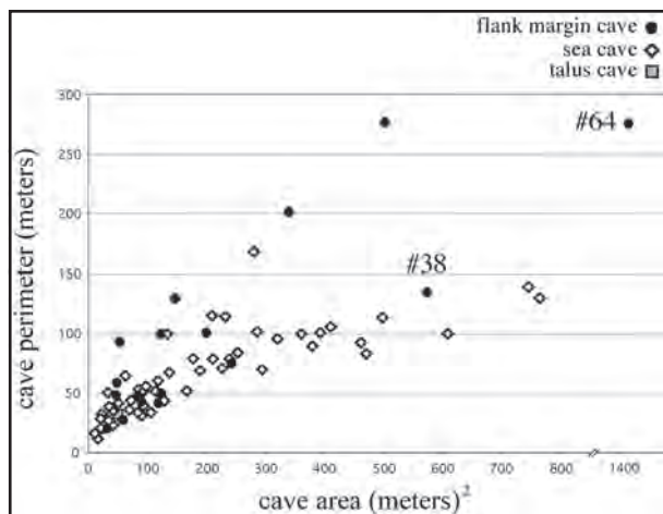
Figure 3: Morphometric differentiation of coastal caves in Puerto Rico. Plot of cave area versus cave perimeter for coastal cave sites with a total area less than 1500 square meters. Flank margin caves are indicated as solid circles, sea caves as open diamonds and talus caves as shaded boxes. Cave sites #38 and #64 indicate flank margin structures modified by significant littoral overprinting.
