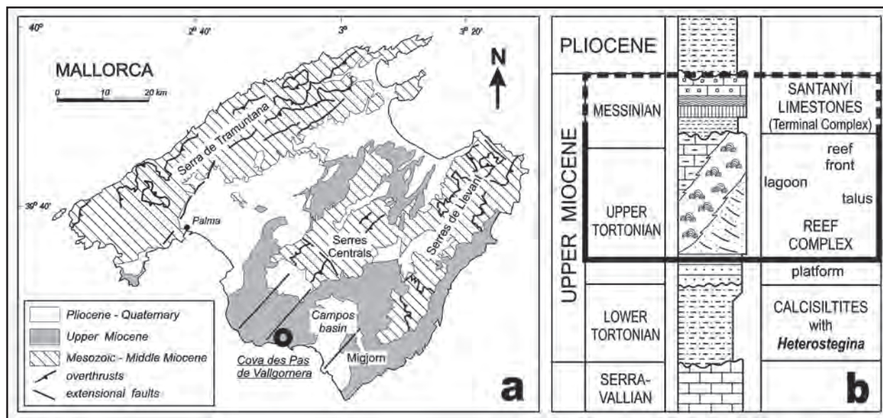
Figure 1: Simplified geological map of the island with the location of the caves (a) and synthetic litho-stratigraphical column of the Upper Miocene in Mallorca (b). The geological units where the endokarst of Migjorn region is developed are highlighted in grey.
