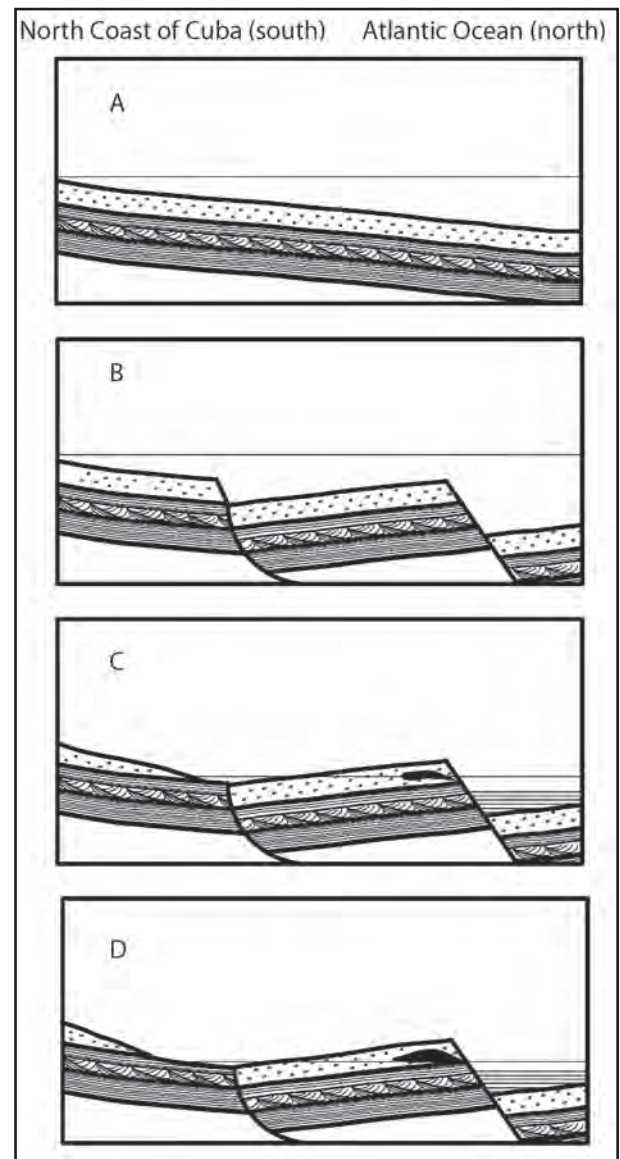
Figure 6: Tectonic evolution of the north coast of Cuba and the development of flank margin caves. A. Shallow, high energy shelf. B. Tectonics caused rotation along east-west trending normal faults resulting in the southward tilting of large structural blocks. C. The upper tips these blocks became emergent by the Pliocene exposing them to meteoric waters and the development of a fresh water lens and flank margin caves. D. Lowering of sea level drains the caves and exposes the surface of the blocks to denudation processes.
