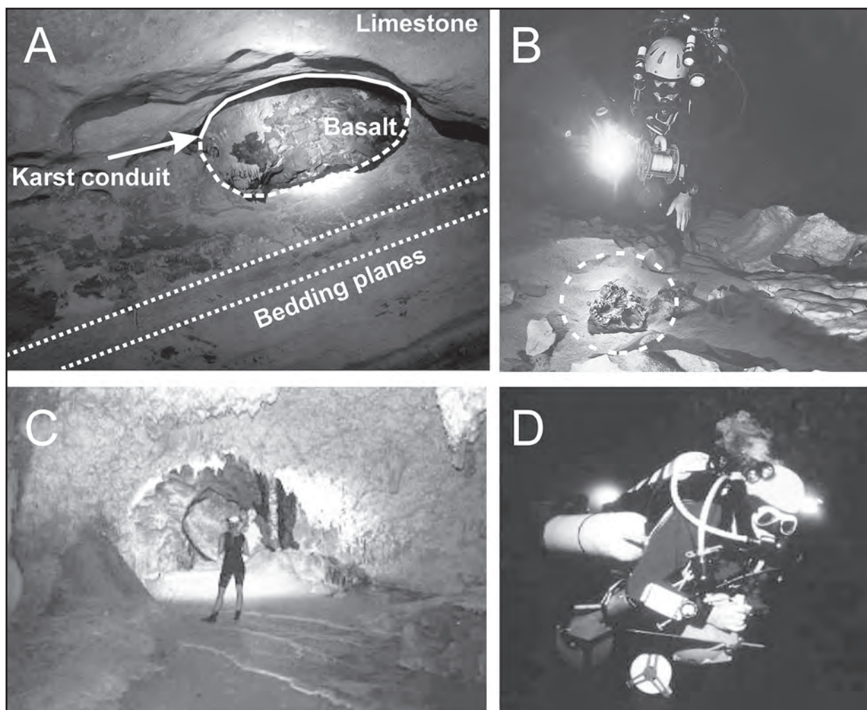
Figure 2: The caves: (A) Basalt (black) filling an ancient karst conduit in the southern branch of Bue Marino cave; (B) Monk seal skull (circled) in a submerged side branch of Bel Torrente cave, at -7 m water depth; (C) The fossil part of Fico cave; (D) Cave diver with complete equipment.
