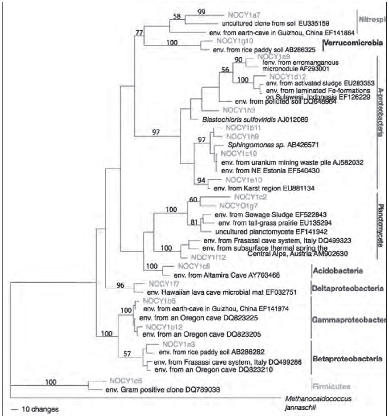
Figure 2: Parsimony tree of bacterial clone sequences from blue-green deposits in Maelstrom lava tube on the big island of Hawai'i. Numbers on the branches indicate bootstrap values from 1000 replicates and indicate the degree of support for relationships within this tree topology.
