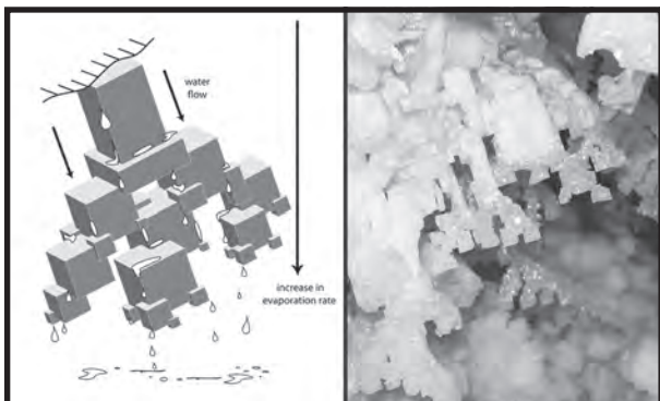
Figure 4: Bi-dimensional pyramid-like monocrystalline trays develops where the dripping is fast and the evaporation rate suddenly increases due to a "sheet" air flow.
