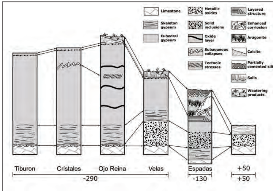
Figure 2: Stratigraphic sketch of the chemical deposits present in each of the Naica caves and their relationships: the deposition sequences are different from cave to cave but many of the in-volved processes are the same, and it was possible to correlate most of them (see arrows) (after FORTI 2009, modified).
