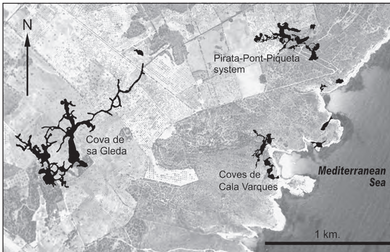
Figure 6: Plotting of the main caves located in Cales de Manacor area. Ramiform patterns are dominant, lacking apparent direct drainage towards the sea.
