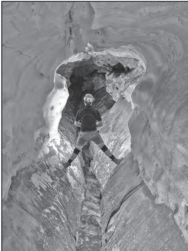
Figure 4: Cross-section of a structurally controlled passage in the upper level of the cave. The joint controlling the passage is clearly seen in its ceiling and corrosion forms can be distinguished at the back of the photo. The upper third of the gallery shows the smoothness of dissolutional morphologies.
