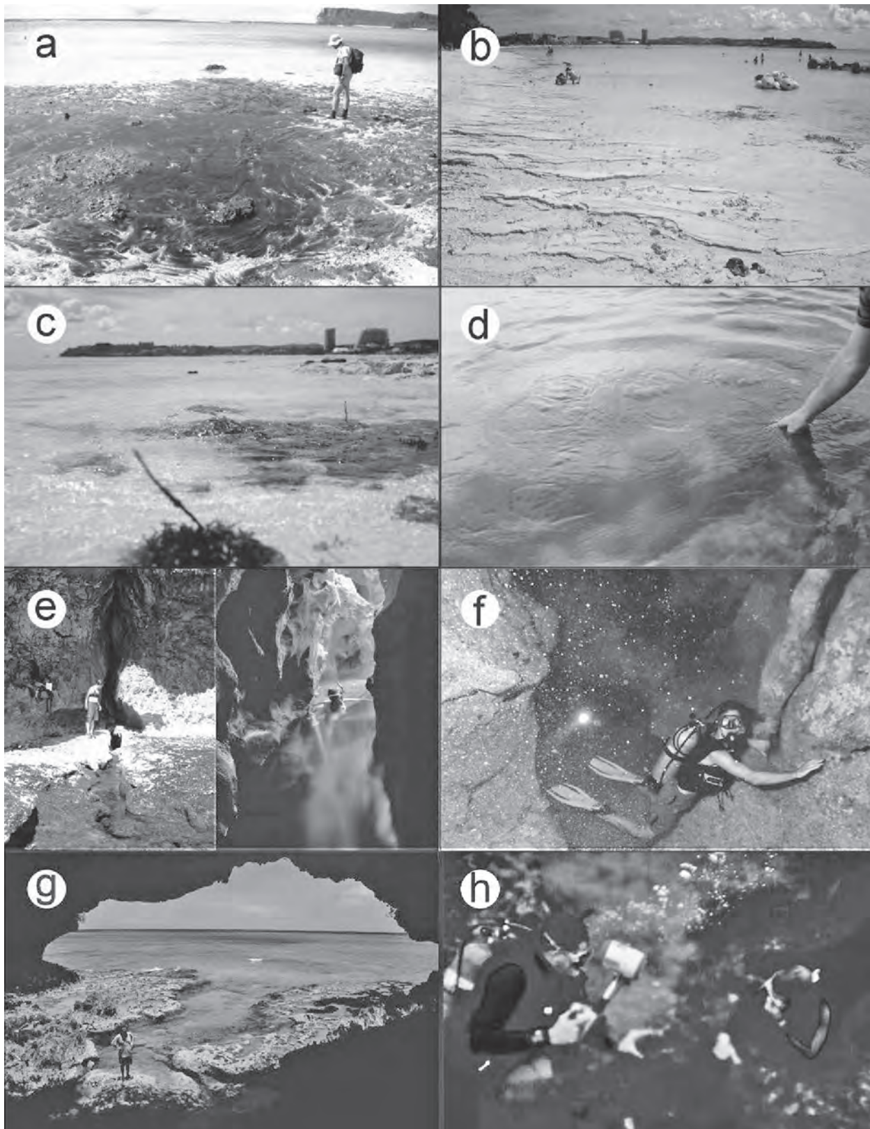
Figure 3: Different types of coastal discharge features in northern Guam. (a) beach seep zone where no distinct point of discharge can be observed, (b) beach springs at low tide, (c) beach spring at high tide, (d) reef spring, (e) fracture spring (outside and inside), (f) submarine fracture spring, (g) cave spring, (h) submarine cave spring.
