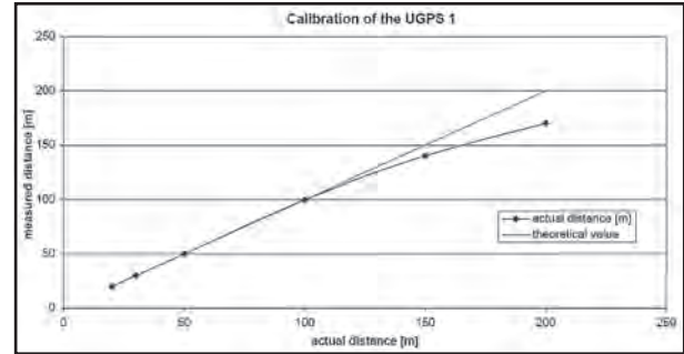
Figure 2: Calibration of the distance indicated by the instrument.
