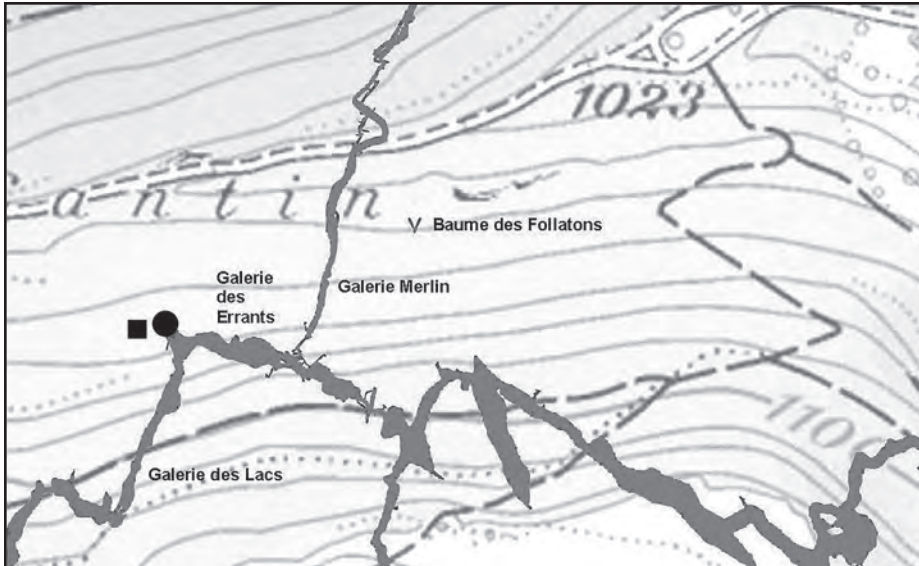
Figure 4: Measurements undertaken in the Grotte aux Fées. The cave survey could be controlled. The indicated depth seems very reasonable (107 m instead of 105 m expected).
