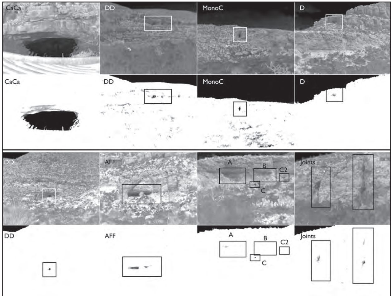
Figure 2: Thermal images of karst features taken from 3:55 to 4:33 P.M., July 15, 2008. The temperature was 36° C and the relative humidity was 34%. The top and third rows are scaled to a temperature range of 20–45° C. The second and bottom rows of images are identical to the top and third except that the images were scaled to a temperature range of 26.5–30° C.
