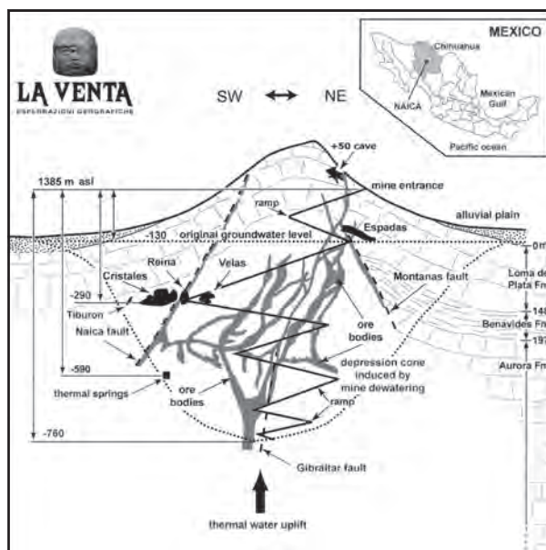
Figure 1: Sketch of the Naica mine in which the largest natural cavities, closely connected to the main faults, are related to the original groundwater level. On the right the stratigraphic sequence is derived from several drilled cores within the Naica Ridge (after FORTI 2009, modified).
