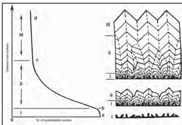
Figure 2: Growth of a parallel-columnar aggregate (from Grigor'ev, 1961). The dissymmetry of geometric selection changes spherical to cylindrical symmetry.
