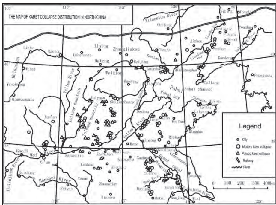
Figure1.:The Paleo-karst collapse pillar distribution in north China.
