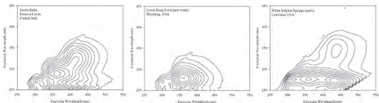
Figure 3. Representative fluorescence spectra of microbial mat waters. The EEMs are interpreted like topographic maps, with tight contours representing steep curves and closed contours being peaks.
