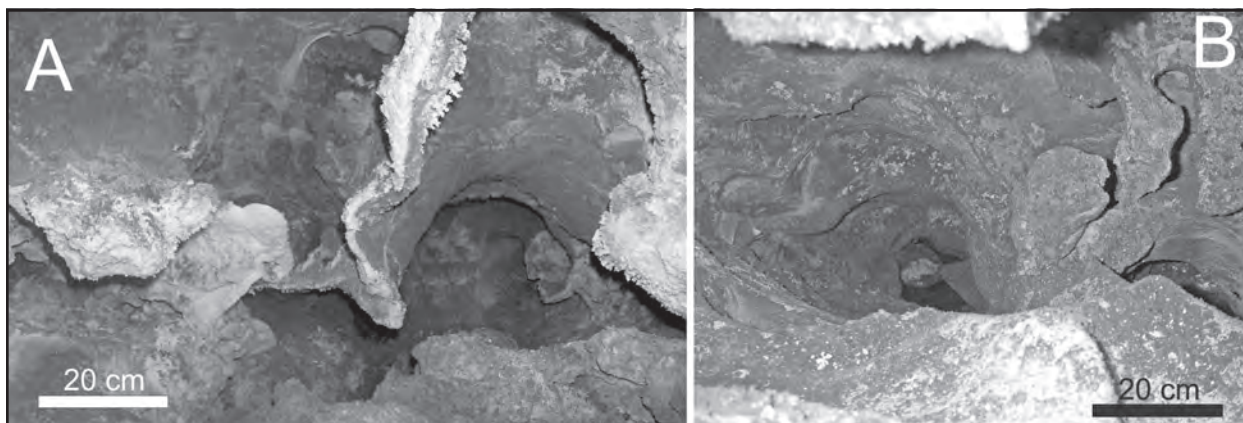
Figure 2: Innermost section of the vent (840–841), showing the walls and ceiling densely covered in multicolored deposits.
