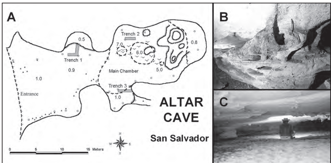
Figure 1: Altar Cave, San Salvador Island, Bahamas. (A) Map of Altar Cave (modified from Florea et al., 2004). Numbers on the floor of the cave are ceiling heights in meters. (B) Speleogens in the wall of Altar cave, at the location of “trench 3” on the cave map shown in A. Pencil in upper right is 15 cm long for scale. (C) Entrance passage of Altar Cave, the site marked “trench 1” on the cave map in A is to the left of the seated figure.
