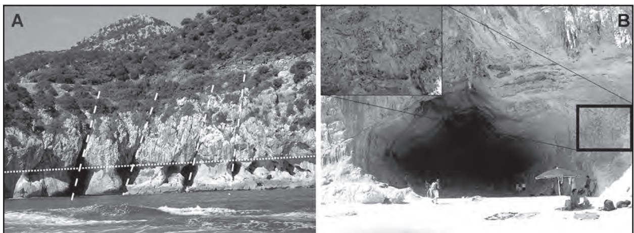
Figure 3: Influence of sea level and fractures on cave development: (A) Coastal caves South of Cala Fuili, with Tyrrhenian notch at 10 m asl. (dotted line) and enlargement of fractures (hidden vertical lines) mainly by mechanical erosion; (B) Cala Luna cave with tidal notch at 9 m asl., two fractures guiding the coastal cavern development. Inset shows Lithophagae holes enhancing notch formation.
