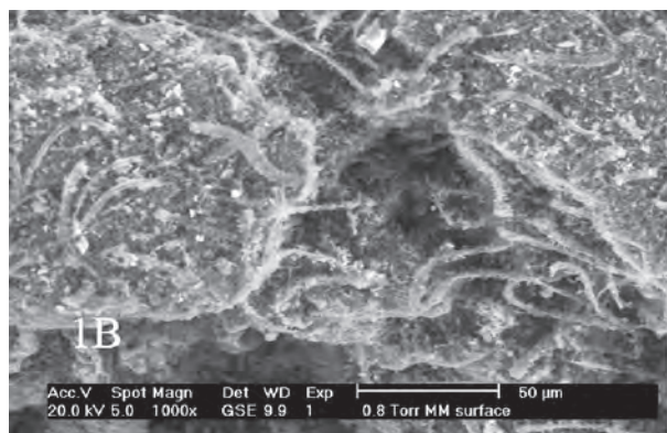
Figure 3: SEM photomicrographs of microbial cells intermixed with carbonate minerals from moonmilk in Grotta della Foos (1B), microbial cells from the moonmilk-water interface in Grotta della Vecchia Diga (2B).
