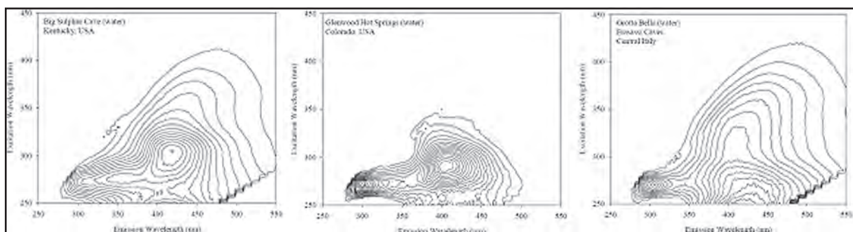
Figure 2. Representative spectra of waters from karst caves and springs. The EEMs are interpreted like topographic maps, with tight contours representing steep curves and closed contours being peaks.
