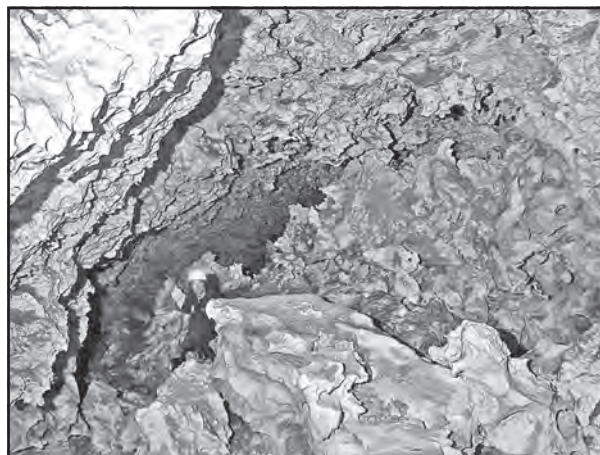
Figure 3: Massive spongework that covers the roof, walls and floor of Galeria del Mig Quilòmetre.
