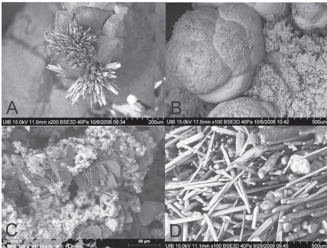
Figure 5: SEM images of some minerals present in the cave rims and vents of Cova des Pas de Vallgornera: (A) strontianite, (B) huntite, (C) nordstrandite, and (D) gypsum needles.
