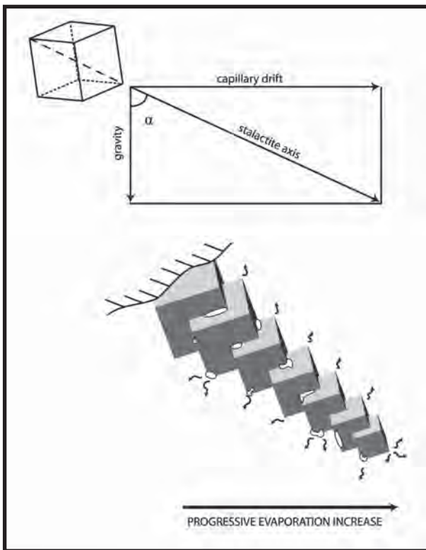
Figure 2: In the presence of an air-flow gradient with a horizontal component and no active dripping, the growing axis of the macrocrystalline stalactite has a direction that corresponds to the vectorial sum of gravitational and capillary flows (top).
