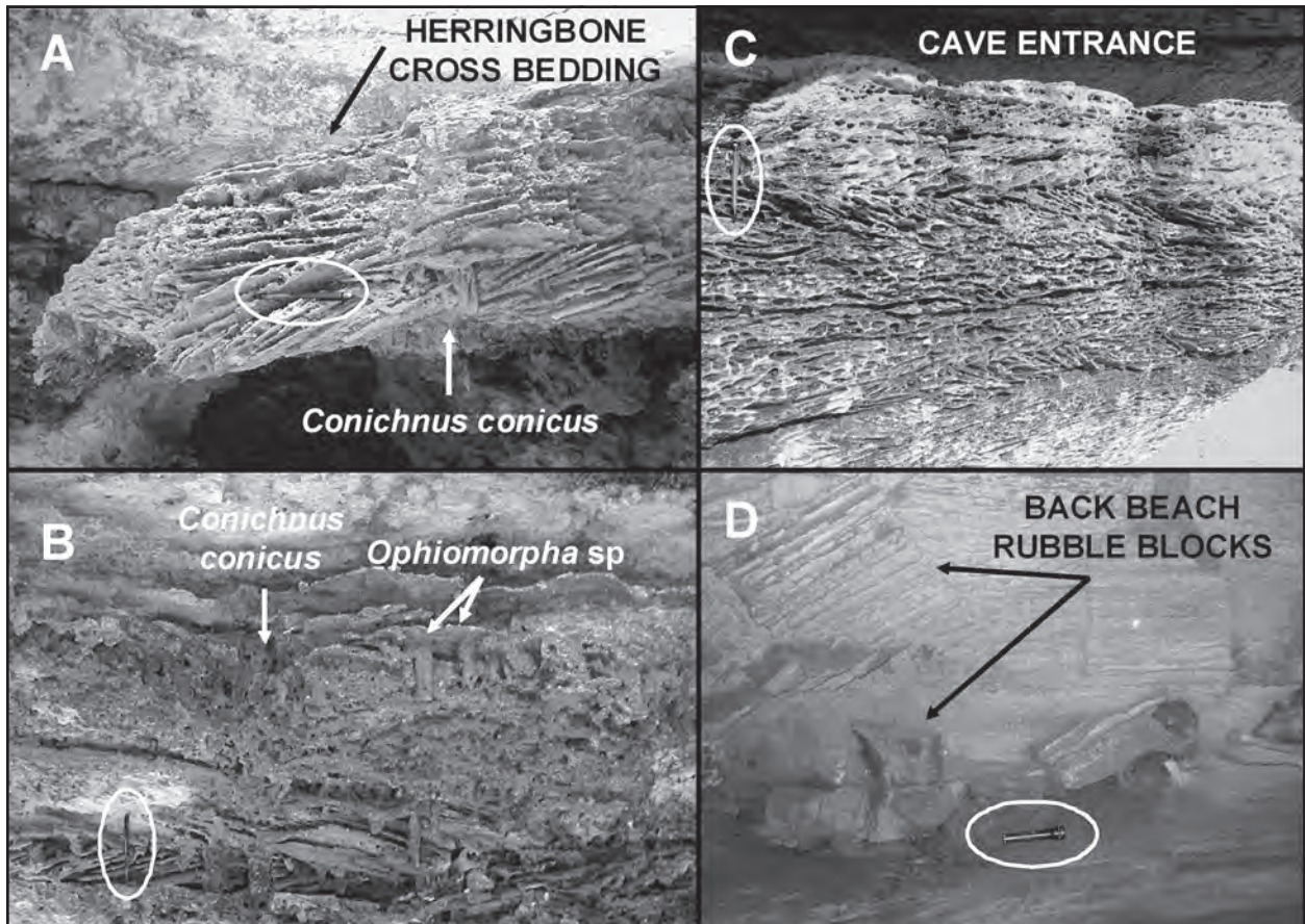
Figure 4: Detail of bedrock walls of Bahamian syndeositional caves, showing numerous subtidal indicators. Pencil in oval in images A-C is 15 cm long, the flashlight in D is 15 cm long, for scale. (A) Cave wall in A-Survey Cave. Herringbone cross bedding, a subtidal indicator, and the subtidal trace fossil Conichnus conicus , the trace left by a sea anemone as it moves upward through sand as the sands cover it, are present. (B) Cave wall in A-Survey Cave. Herringbone cross bedding is visible in the lower left near the pencil. Conichnus conicus is present, as is Ophiomorpha sp, the trace of a subtidal burrowing shrimp. (C) Cave wall at lower entrance to Chinese Fire Drill Cave, showing herringbone cross bedding. (D) Cave wall at the Pink Grotto, adjacent to Altar Cave, showing back-beach breccia blocks above subtidal sands with herringbone cross bedding, and below overlying back-beach calcarenites.
