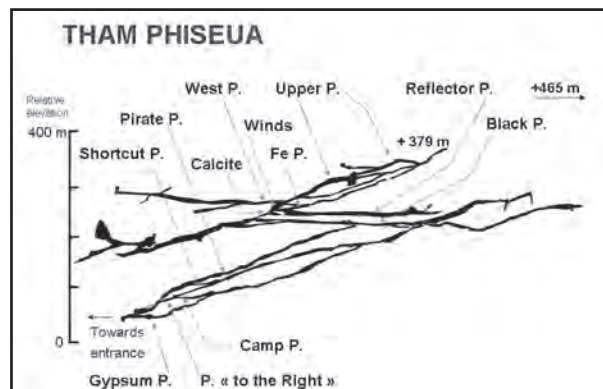
Figure 1: Schematic long cross-section of the sampled part of the hypogenic passages of Tham Phiseua (active subhorizontal levels are not shown).
