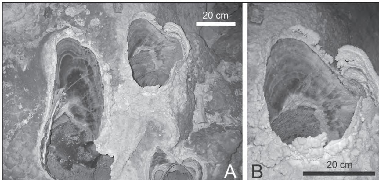
Figure 4: General aspects of large vent related rims; (A) group of three cave rims developed on the gallery's floor; (B) cave rim showing in detail the white crystallizations.
