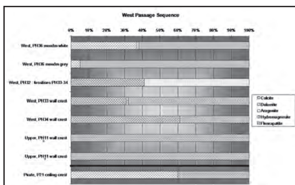
Figure 3: Mineral succession of the main phases (younger on top) in West Passage.
