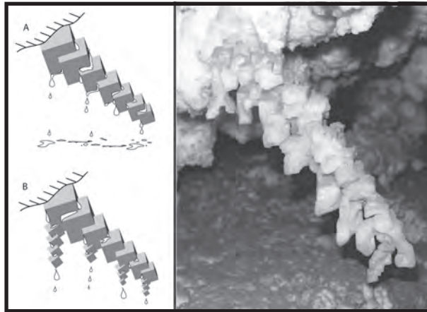
Figure 3: In the presence of an air flow gradient with an horizontal component and an active dripping, new vertical stalactites develop from the lower tips of the crystals by dripping.
