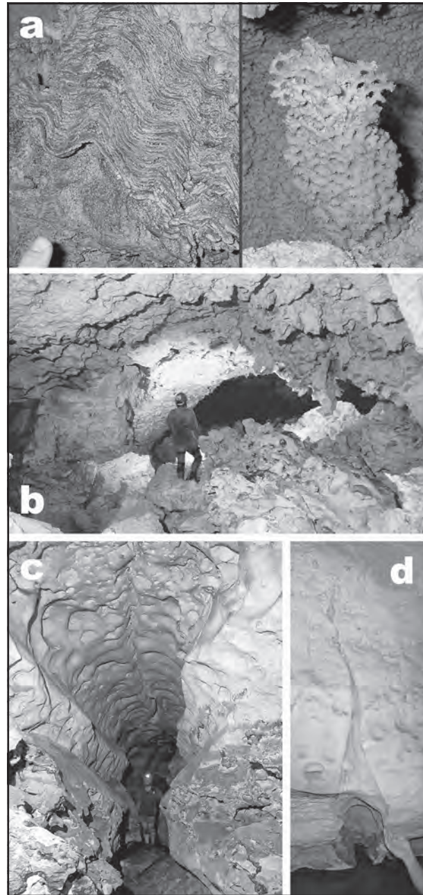
Figure 3: Cova des Pas de Vallgornera; morphological aspects of its passages and chambers. (a) detail views of coral structures affected by solutional processes; (b) the passage called Galeria del Mig Quilòmetre (Sector del Clypeaster) runs over 500 m all along the reef front, without any structural control and showing spectacular dissolution features on its whole cross-section; (c) view of a joint-guided gallery developed in the outer lagoon facies and shaped with spectacular dissolution features (notches, bevels, pockets of diverse size...); (d) conspicuous solutional rising channels, of a possible hypogenic origin, are well-represented particularly in the passages from Sector de Gregal (Photos: Antoni Merino).
