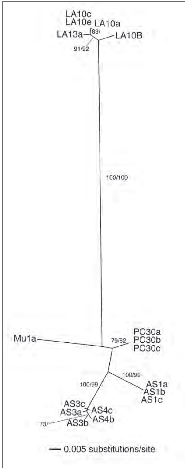
Figure 3: Unrooted neighbor joining tree of ITS sequences from Acidithiobacillus isolates. Sequences are coded by location as follows: AS = Rio Garrafo (Italy), Mu and PC = two different locations within Frasassi (Italy), LA = Luna Azufre (Mexico). Bootstrap values for neighbor joining and maximum parsimony greater than 50 are shown for each node. Note the significant separation among sequences from different Italian samples.
