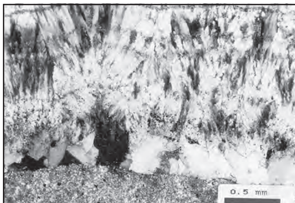
Figure 1: As the supply solution becomes more saturated, the spar crystals at the base of this flowstone change to split coconut-meat crystals. Photo V. Polyak.
