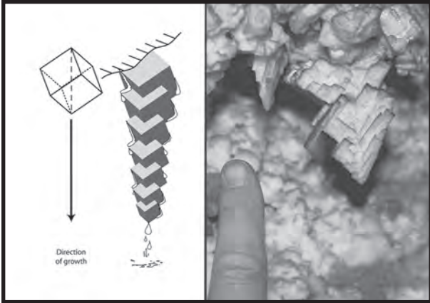
Figure 1: Evolution of a vertical halite macrocrystalline stalactite: due to the competitive growth the interpenetrated cubes have their long diagonal coincident to the stalactite axis which is parallel to the vertical. Verticality is also maintained if the water supply is only by capillarity in absence of an air flow gradient with a horizontal component.
