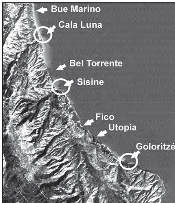
Figure 4: Landsat TMS image, band 1 (December 23, 1998) with the major cave systems indicated. The circled areas correspond to sea water transparency indicating fresh water outflows.
