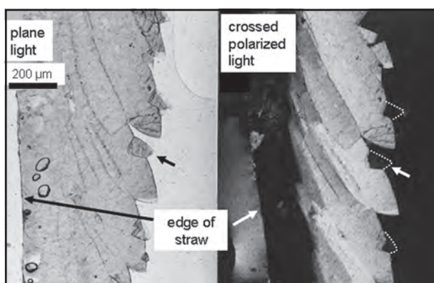
Figure 2: Thin section micrograph of the wall of a soda straw from Hell Below Cave. The image on the left shows large subcrystals splitting from a larger composite crystal. The arrow points to a growth hillock on one of these subcrystals. The image on the right is viewed through crossed polarizers and shows different shades of gray representing varying degrees of orientation caused by crystal splitting. White arrow points to growth hillocks that are optically extinct under crossed polarizers.
