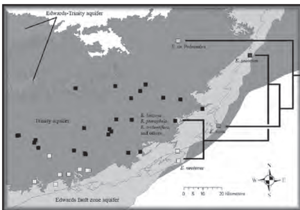
Figure 3: Relationships among the major groups of the southeastern Blepsimolge and their distribution with respect to the major aquifers of the Edwards Plateau.
