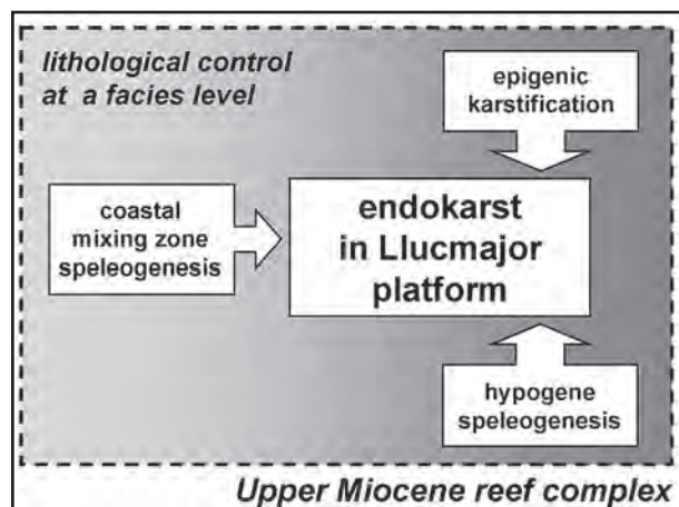
Figure 4: The genesis of Cova des Pas de Vallgornera is a complex matter owing to the confluence of three speleogenetic vectors that have acted altogether, but conditioned by strong lithological factors.
