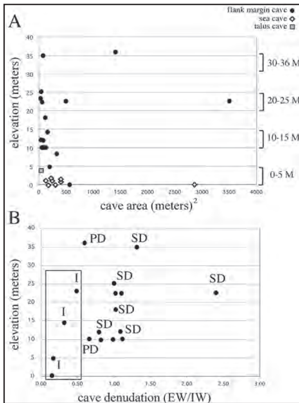
Figure 5: (A) Plot of total cave area versus cave elevation (relative to contemporary mean sea level). Flank margin caves are indicated as solid circles, sea caves as open diamonds and talus caves as shaded boxes. (B) Plot of degree of Cave Denudation (the ratio of maximum entrance width to maximum internal width) versus cave elevation in meters for the flank margin cave data set, where I = intact structure, PD = partially denuded and SD = significantly denuded.
