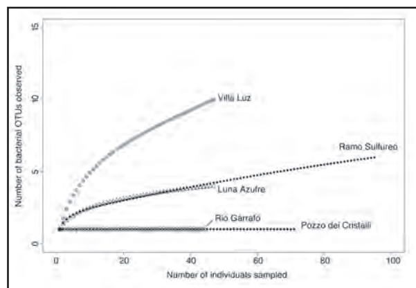
Figure 1: Rarefaction curves for 16S rDNA bacterial clone libraries from five snottite samples. Operational taxonomic units (OTU's) are defined by 98% sequence similarity.
