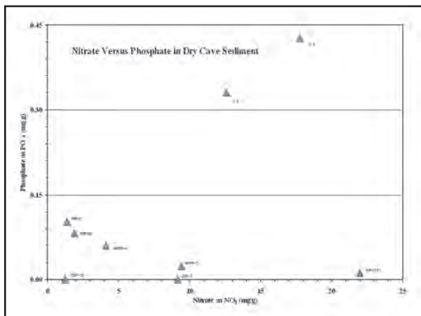
Figure 2: Plot of nitrate and phosphate concentrations in dry cave sediments.
