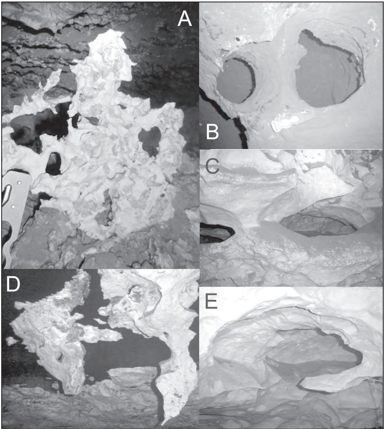
Figure 4: Several examples of corrosion morphologies (microforms) related to the coastal mixing zone from Cova des Coll (eastern Mallorca): (A) spongework; (B) arches; (C) wall pockets; (D) rock pendants and (E) rock jags.
