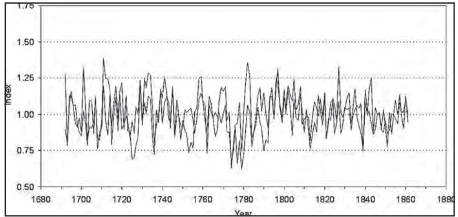
Figure 3: Comparison of the Norris Dam State Park white oak reference chronology (gray line) and the Cagle Saltpetre Cave white oak chronology developed by dendrochronological analyses (darker line) (from, BLANKENSHIP et al., 2009: Figure 5).
