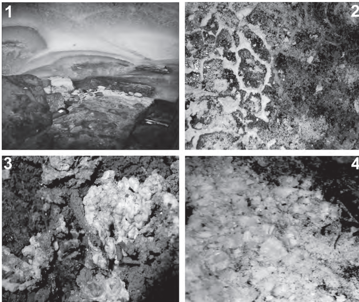
Figure 2: Gypsum powder forms: 1, accumulation of powder under the naled ice between Diamond and Polar Caves, 2, powder remnants on the spot of the melted seasonal ice form, 3, initial aggregation (sticking and crystallization) of cryogenic “remnants,” 4, gypsum crystals growing from the cryogenic gypsum material (1, photo V. Andreychouk, 2–4, O. Kadebskaya).
