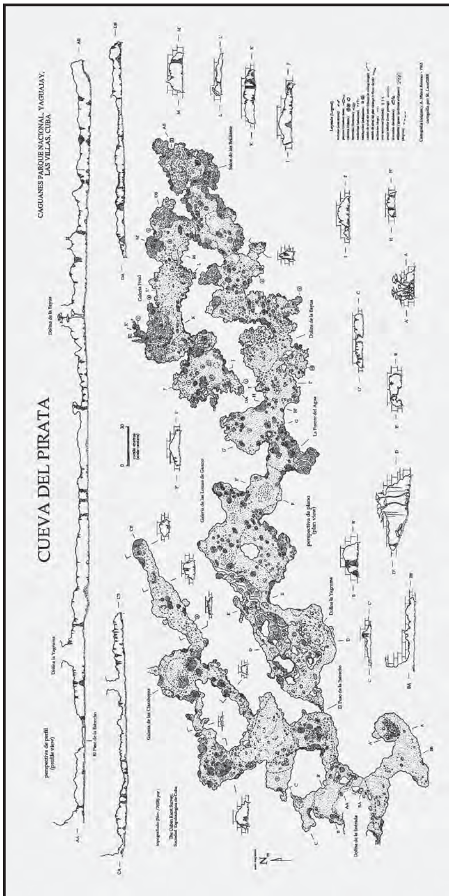
Figure 4: Typical flank margin cave on Cayo Caguanes.
