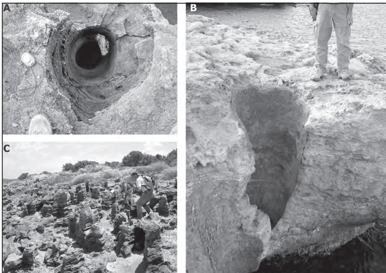
Figure 1: Dissolution pipes: (A) A dissolution pipe with calcrete lining at Punta Funtanas (Sardinia); (B) Dissected pipe with calcrete lining at Roca Vecchia (Apulia); (C) a “field” of pipes along the Tabarka coast (Tunisia).
