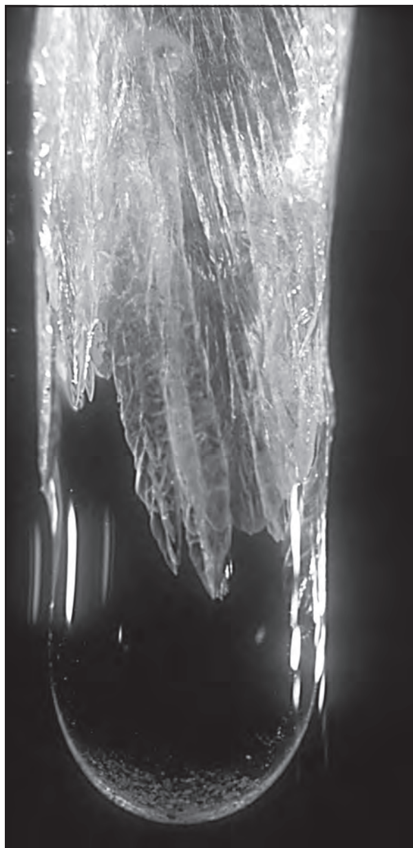
Figure 4: The drip point of a stalactite, with a crown of skeleton crystals. Photo V. Maltsev
