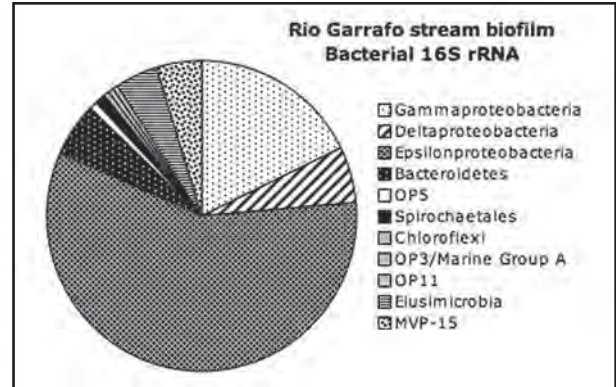
Figure 2: Taxonomic composition of bacteria in Rio Garrafo stream biofilms collected in 2005 and 2007. A total of 174 clones are represented. The composition of the two libraries is similar. Major lineages were identified by sequence analysis using the software program ARB. Most lineages are represented in the libraries by a single phylotype (> 98% sequence similarity). Exceptions are annotated with the number of phylotypes on the diagram.
