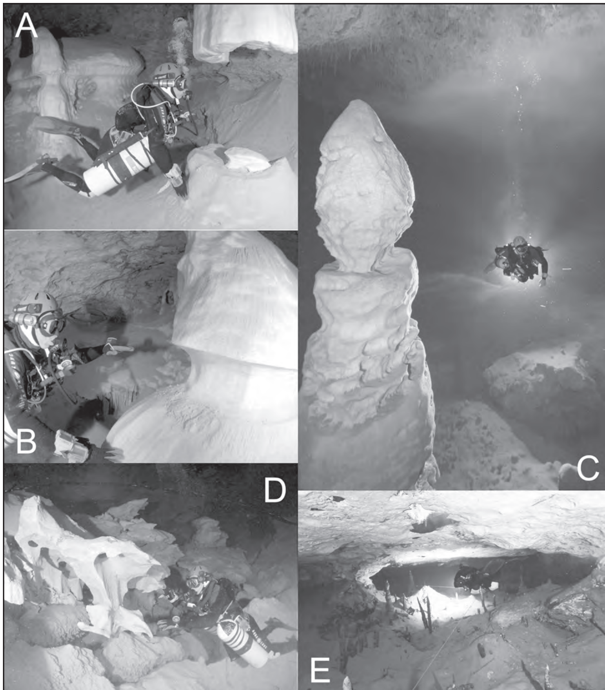
Figure 3: Several examples of corrosion morphologies (macro- mesoforms) related to the coastal mixing zone from Cova de sa Gleda (eastern Mallorca): (A) column sectioned by water dissolution; (B) notch; (C) column affected by an important narrowing caused by the dissolution in the mixing zone; (D) spongework morphologies; and (E) phreatic gallery with elliptical section.
