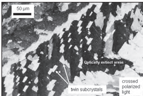
Figure 6: Thin section micrograph viewed through crossed polarizers showing multiple growth hillocks in fibrous surface-travertine calcite from Sitting Bull Falls.
