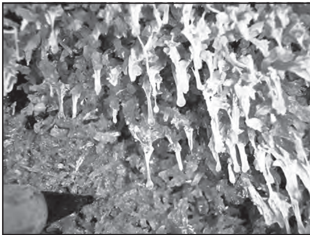
Figure 1: Rio Garrafo snottites developed on the surface of calcium sulfate (selenite) crystals. The crystals and associated acidic biofilms coat the limestone walls of the cave where sulfidic vapor rises from the water table. Pencil at lower left for scale.
