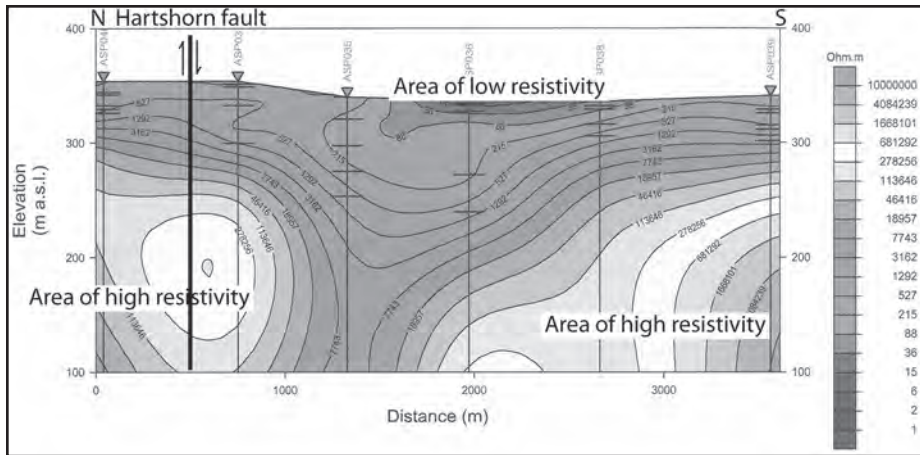
Figure 8: Audio-magnetotelluric and topographic profile line "Western Trace". See Figure 4 for line and station locations. 3X vertical exaggeration.
