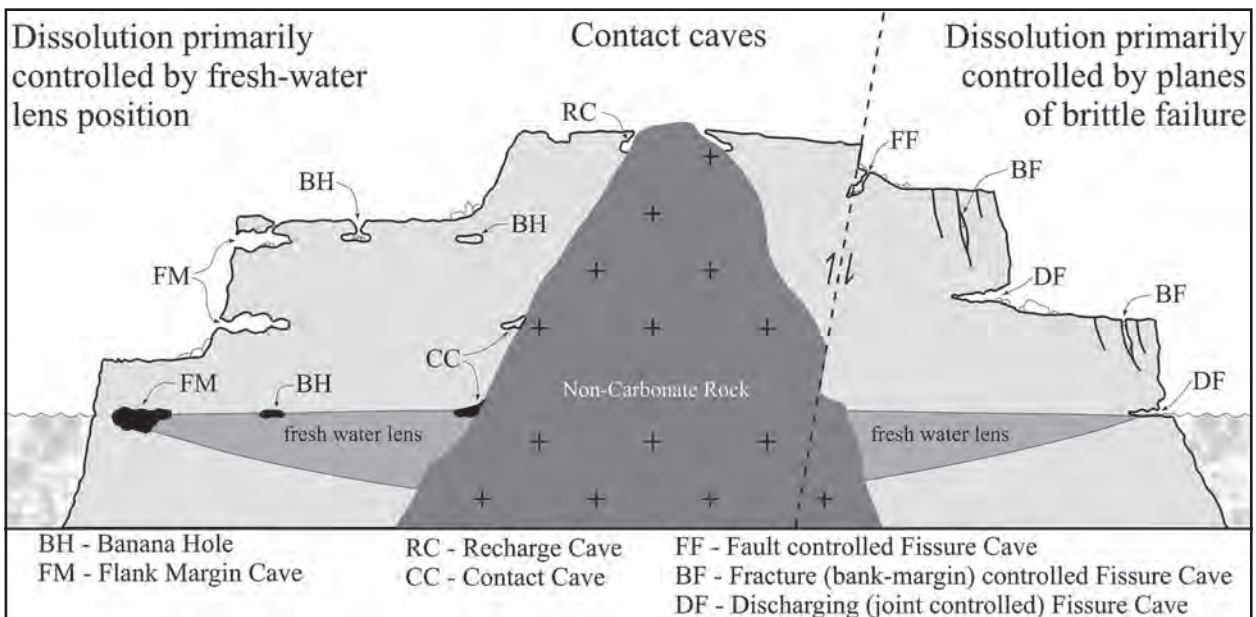
Figure 2: Schematic diagram depicting the different types of caves that are commonly encountered in the Northern Mariana Islands (adapted from Stafford et al., 2005).
