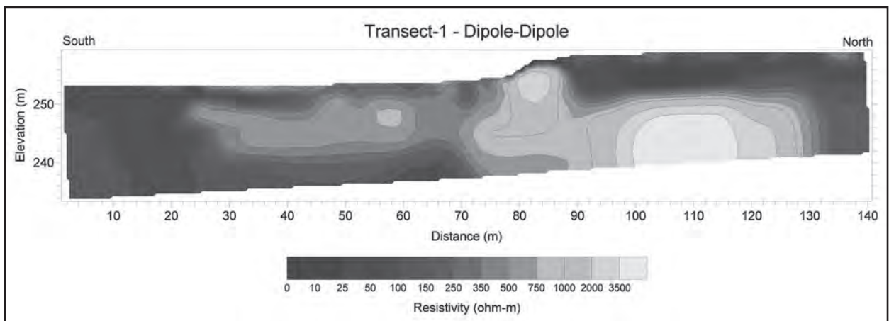
Figure 3: Vertical cross sections of electrical resistivity collected with a dipole-dipole array (top). Lower resistivity is denoted by dark colors and is interpreted to be surface soil or shale- or marl-rich limestone. Higher resistivity is denoted by light colors and is interpreted to be a massive limestone. The highest resistivity is denoted by white and is interpreted to be a potential solution cavity.
