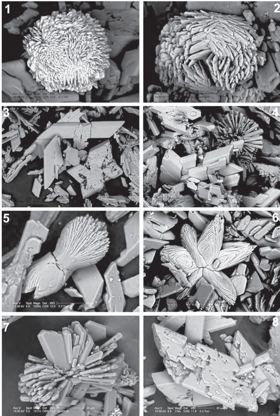
Figure 3: Morphology of crystal aggregates: 1–2, split spherulitic aggregates of celestine, 3–4, tabular and platy gypsum crystals, 5–6, rose-like and sheaf-like calcite crystals, 7, spherulitic gypsum crystal aggregates, 8, skeletal gypsum crystals.
