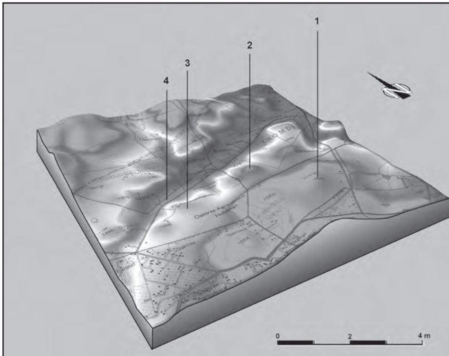
Figure 4: 3D view of the Blauwbankspuit valley around the Sterkfontein area showing the different horizontal surfaces: 1: The highest (around 1580 m of altitude); 2: Between 1,500 and 1,510 m; - 3: Large shelf, well preserved with laterite (1,480 m); 4: Lower shelf, covered with alluvium, a few meter above the river.
