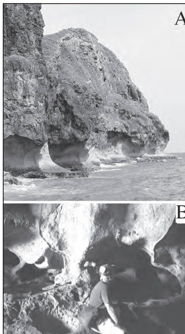
Figure 1: (A) Littoral erosion of northern escarpment of Puerto Rico. (B) Characteristic complex cusped morphology of a flank margin cave perimeter, Cueva Hermina Grande, northern coastline.
