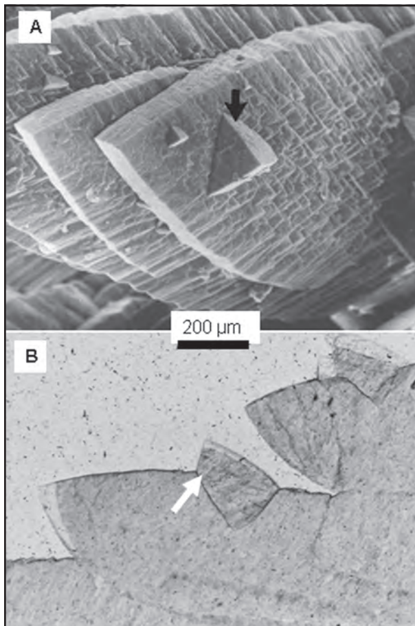
Figure 5: A closer look at leaf-shaped subcrystals. (A) A SEM image showing growth hillocks on surface of leaf-shaped subcrystals. (B) Thin section micrograph showing section through subcrystal and hillock. Each leaf-shaped subcrystal is a distorted rhomb (faces of the rhomb are rough and curved). Twinning expresses itself as growth hillocks (arrows in both A and B).
