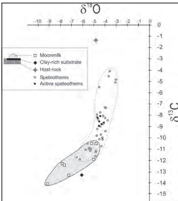
Figure 1: Plot of \delta^{13}C - \delta^{18}O for calcitic moonmilk deposits and associated features of Altamira Cave.
