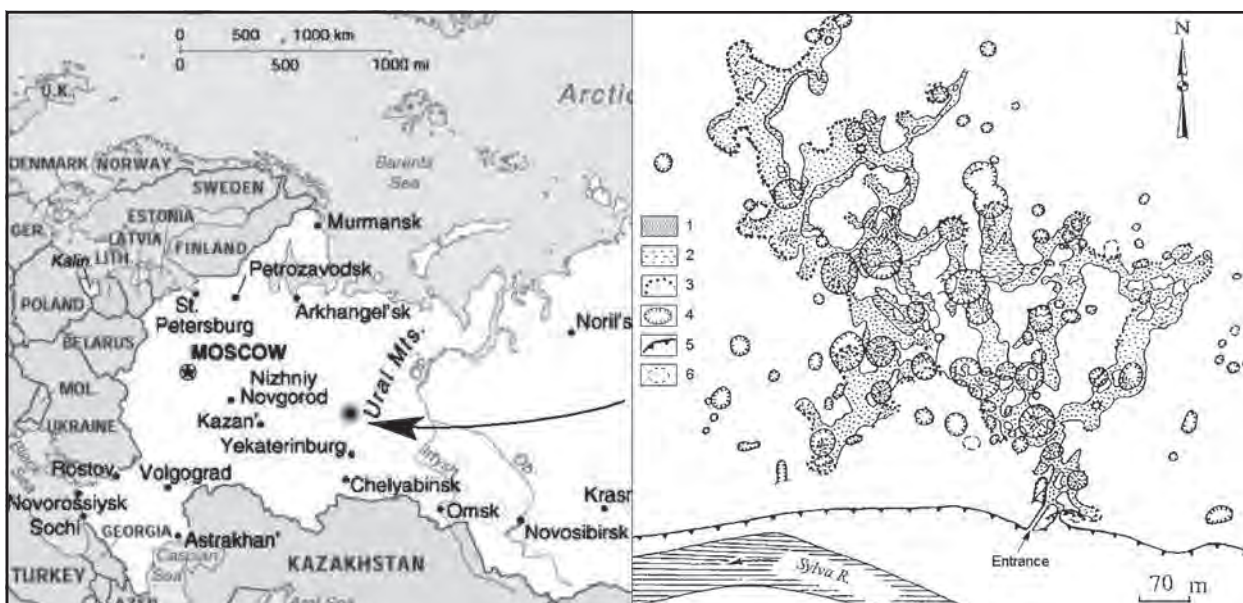
Figure 1: Location of the Koungur Ice Cave and main elements of its underground space: 1, cave space, 2, underground lakes, 3, debris walls and cones, 4, sinkholes, 5, edge of Sylva River Valley, 6, depression of subsidence.
