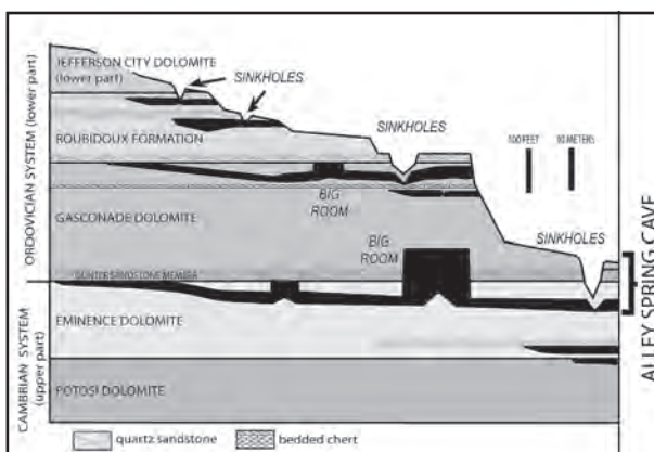
Figure 2: Stratigraphic level of the known part of Alley Spring Cave (black bracket) in relation to a conceptual model of stratigraphic control on cave elevations in the Ozarks of southern Missouri (from ORNDORFF, et al 2006). Note similarity of the known cave profile(Fig.3) to this conceptual model which was originally drawn in 2001.
