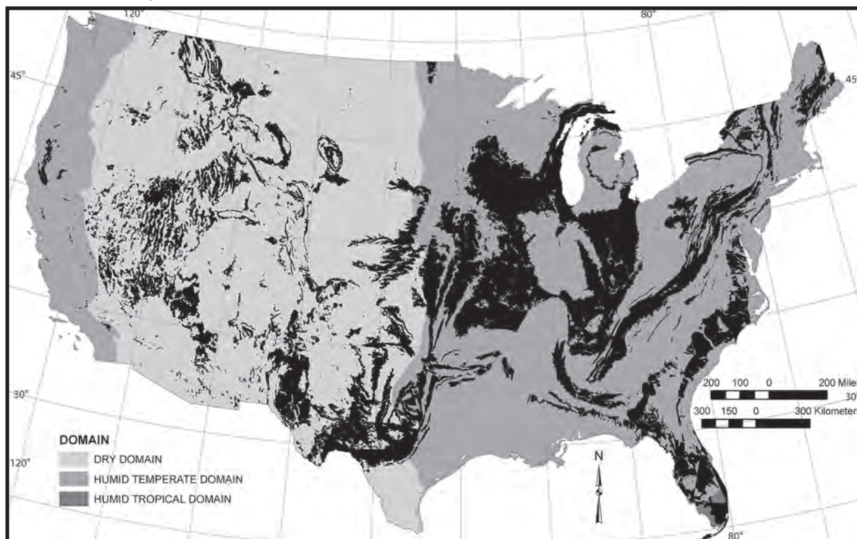
Figure 1: Generalized map of areas of potentially karstic rocks in the conterminous United States. Areas with potential for volcanic pseudokarst also included.
