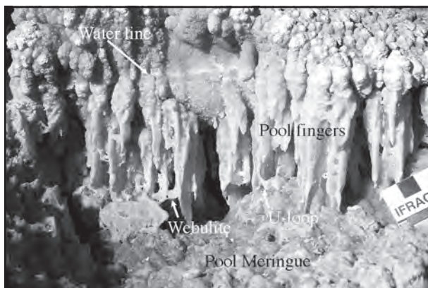
Figure 1: Pool fingers extending down from shelfstone in a paleopool in the Big Room, Carlsbad Cavern. Note that the fingers extend down from the shelf but not from deeper overhangs in the lower left (arrow). Photo by K. Ingham.
