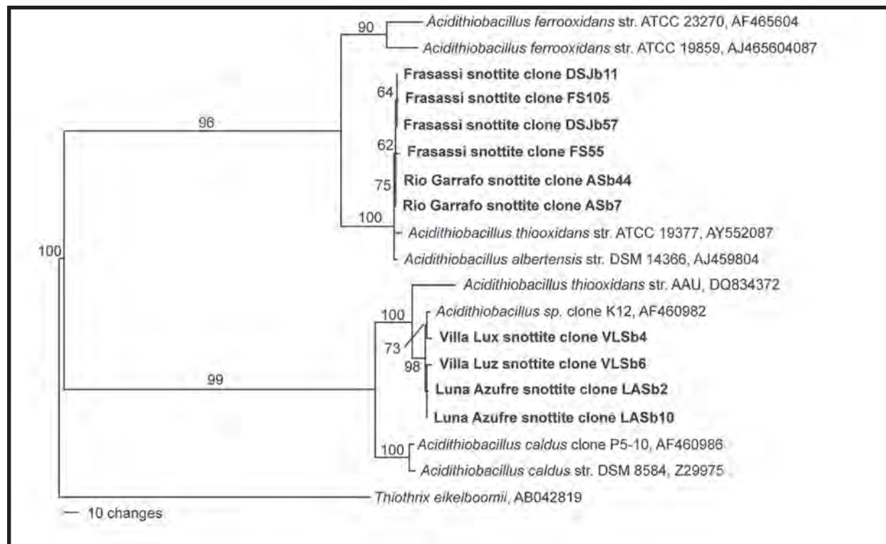
Figure 2: Maximum parsimony phylogenetic analysis of 16S rRNA gene sequences for the bacterial genus Acidithiobacillus . Sequences from this study are shown in bold. Bootstrap values greater than 50 are shown for each node. Note the significant separation between sequences from Mexico and Italy.
