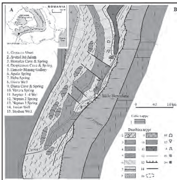
Figure 1: Geologic map of the lower Cerna Valley and location of sampled caves (from NĂSTĂSEANU, 1980); 1: schist (Sebeş-Lotru formation); 2: wildflysch (Upper Cretaceous); 3: Urgonian limestone (Barremian-Aptian); 4: marly-limestone (Iuta formation); 5: limestone (Valanginian-Hauterivian); 6: cherty limestone (Upper Jurassic); 7: detrital limestone (Middle Jurassic); 8: quartz sandstone (Upper Liasic); 9: conglomerate (Lower Liasic); 10: schist (Neamțu formation); 11: Cerna granite; 12: geologic boundary; 13: thrust; 14: fault line; 15: olistolith limit; 16: cave; 17: shaft; 18: mining gallery; 19: thermal water spring; 20: thermal water well.
