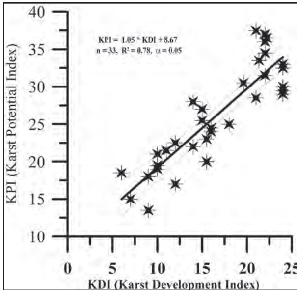
Figure 2: Correlation of the KDI value from composited polygons representing a single stratigraphic unit. A given KPI score may occur for a number of stratigraphic units with a narrow range of KDI score.
