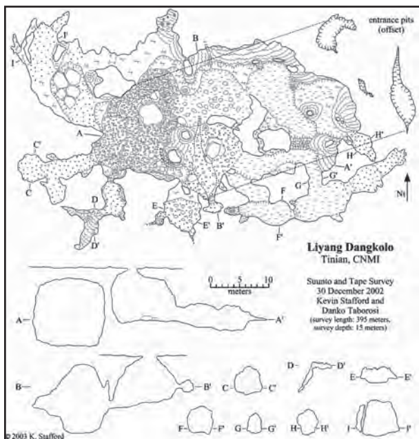
Figure 4: Map of Liyang Dangkolo, a complex flank margin cave on Tinian showing the coalescing of multiple globular chambers (from Stafford, 2003).
