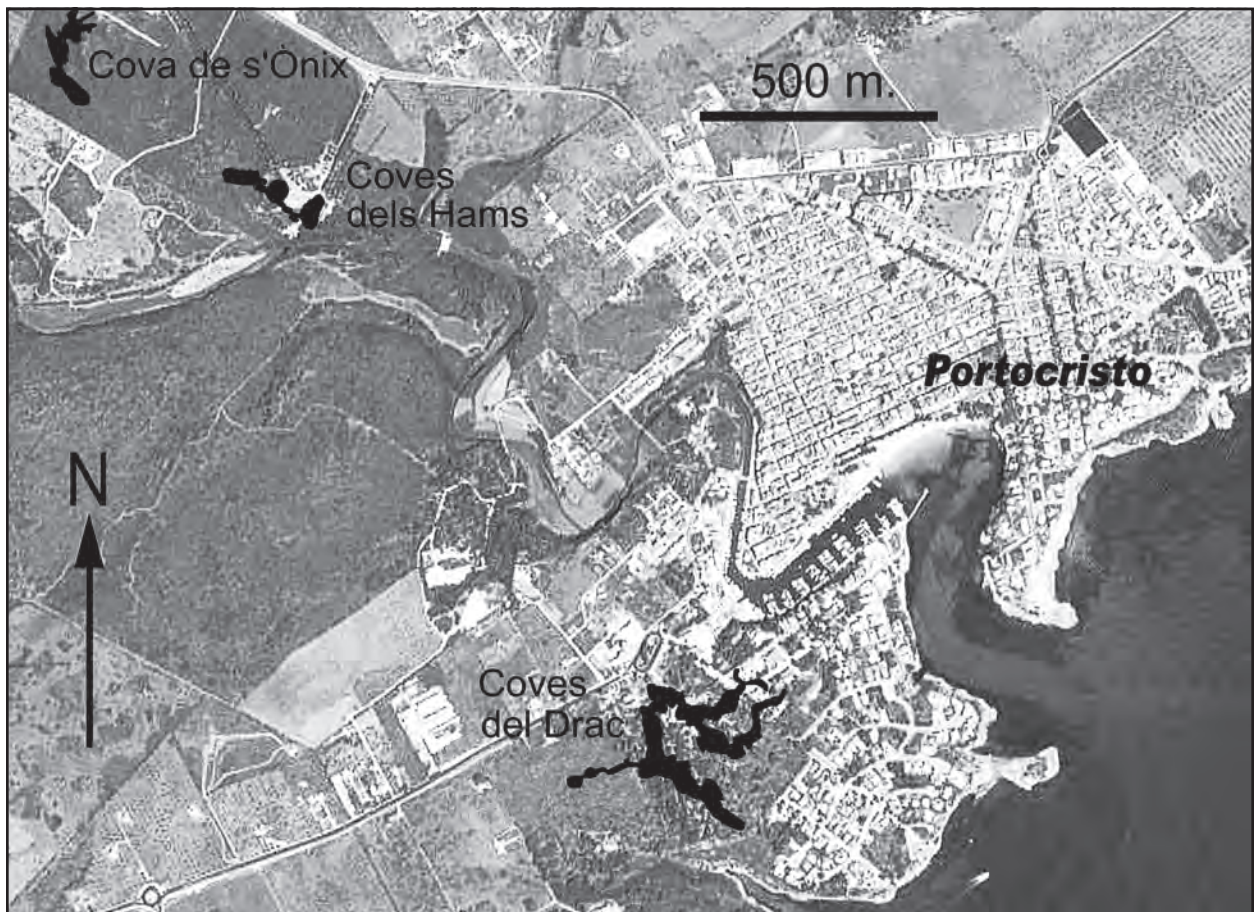
Figure 3: Plotting of the main caves located around Portocristo harbour. Note the wandering trend and the remarkably non-directional path of the celebrated Coves del Drac cavern, placed just between the incised creek of Torrent de ses Tallioles and the small bight of Cala Murta visible at the southern side of the figure.
