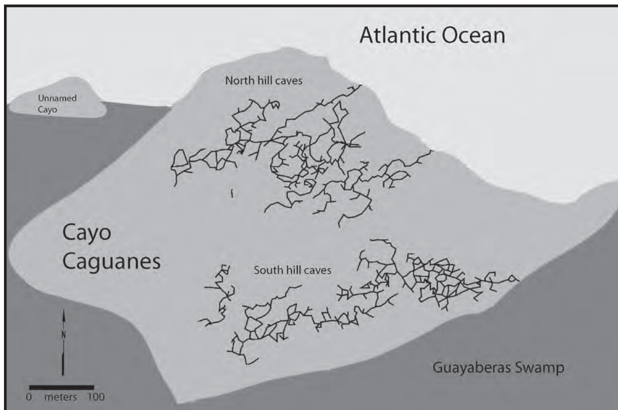
Figure 2: Simplified map of Cayo Caguanes showing current location of flank margin caves with respect to the north and south hills of the cayo.
