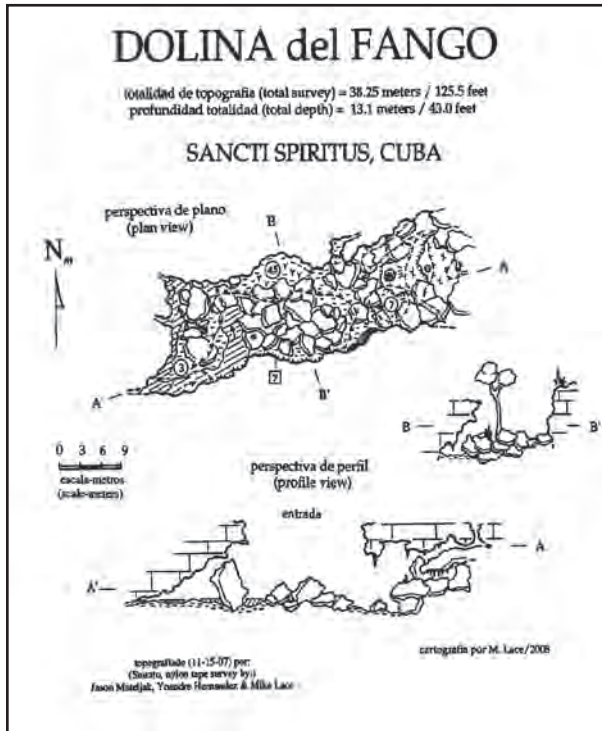
Figure 5: Banana hole on the north hill of Cayo Caguanes.
