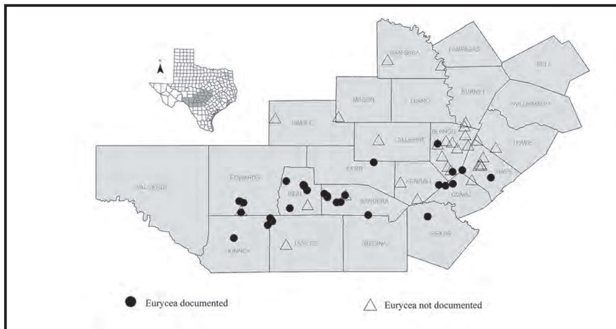
Figure 1: Location of central Texas springs surveyed for Eurycea salamanders.
