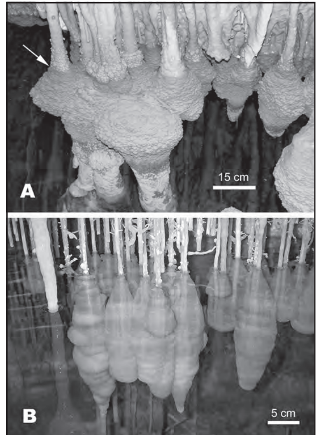
Figure 1: View of the carbonate crystallisations occurring at the surface of brackish pools in the studied caves. A: calcite belt of POS in Cova de Cala Varques A (Manacor). B: aragonite belt of POS from Cova des Pas de Vallgornera (Llucmajor); the thickest part of the overgrowth band corresponds to the mean sea level.
