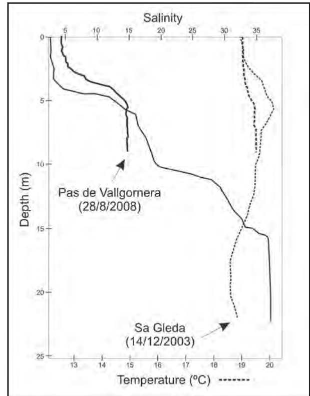
Figure 2: Characteristic temperature and salinity profiles obtained in the brackish water pools located in karstic cavities (Cova des Pas de Vallgornera and Cova de sa Gleda) of the south-eastern area of Mallorca.
