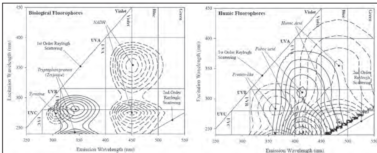
Figure 1. Peak positions for biological (left) and humic fluorophores (right); locations of Rayleigh scattering bands and ultraviolet and visible light regions also shown. Sources for peak positions are cited in the text. The EEMs are interpreted like topographic maps, with tight contours representing steep curves and closed contours being peaks.
