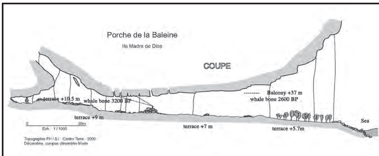
Figure 6: Longitudinal section of Whale Cave with location of marine terraces and radiocarbon datings.
