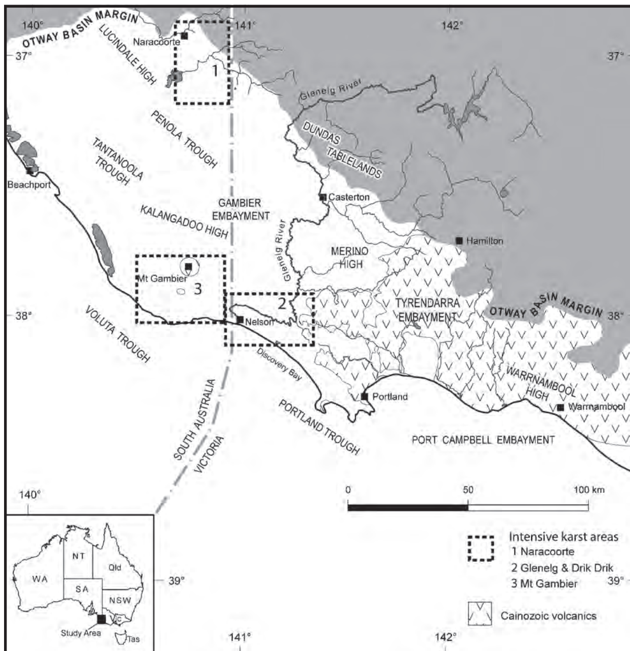
Figure 1: Western Otway Basin and Gambier Karst Province.
