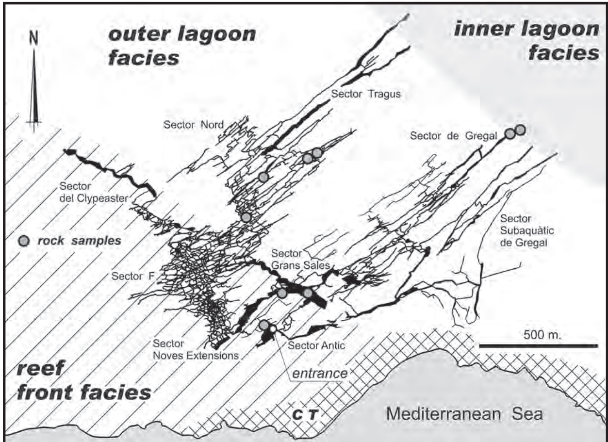
Figure 2: The plan pattern of Cova des Pas de Vallgornera shows clear relations with the facies disposition within the Upper Tortonian Reef Complex in the Lluçmajor platform (southern Mallorca). The Messinian Terminal Complex (CT) outcrops only at the sea cliffs of the area. The location of rock samples used for the lithofacies characterisation is included in the figure.
