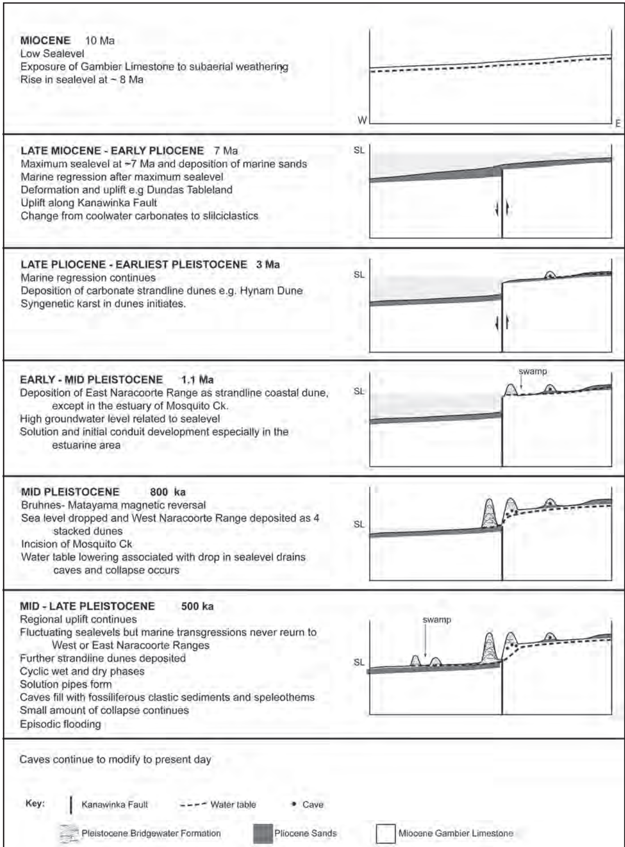
Figure 3: Stages of landscape development, Naracoorte.
