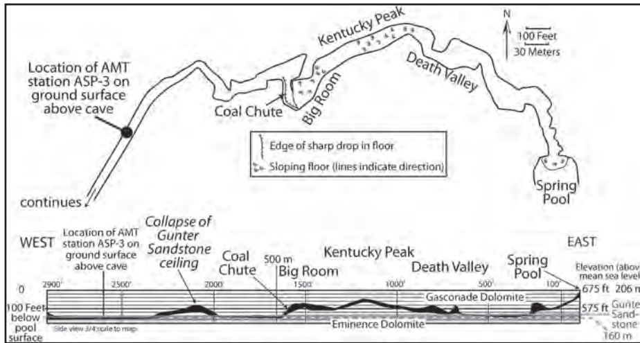
Figure 3: (A) Map and profile of Alley Spring Cave simplified from a map produced by the Ozark Cave Diving Alliance (OCDA, 2005). Geologic interpretation by D. Weary, based on surface geologic mapping, observations by OCDA divers, video footage, and analogy to geologic control seen in air-filled caves in the region. Dashed line indicating 160 m elevation is the level of the electromagnetic resistivity map (Fig. 8).
