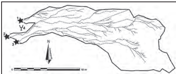
Figure 10: Hydrological catchments and runnel survey.
